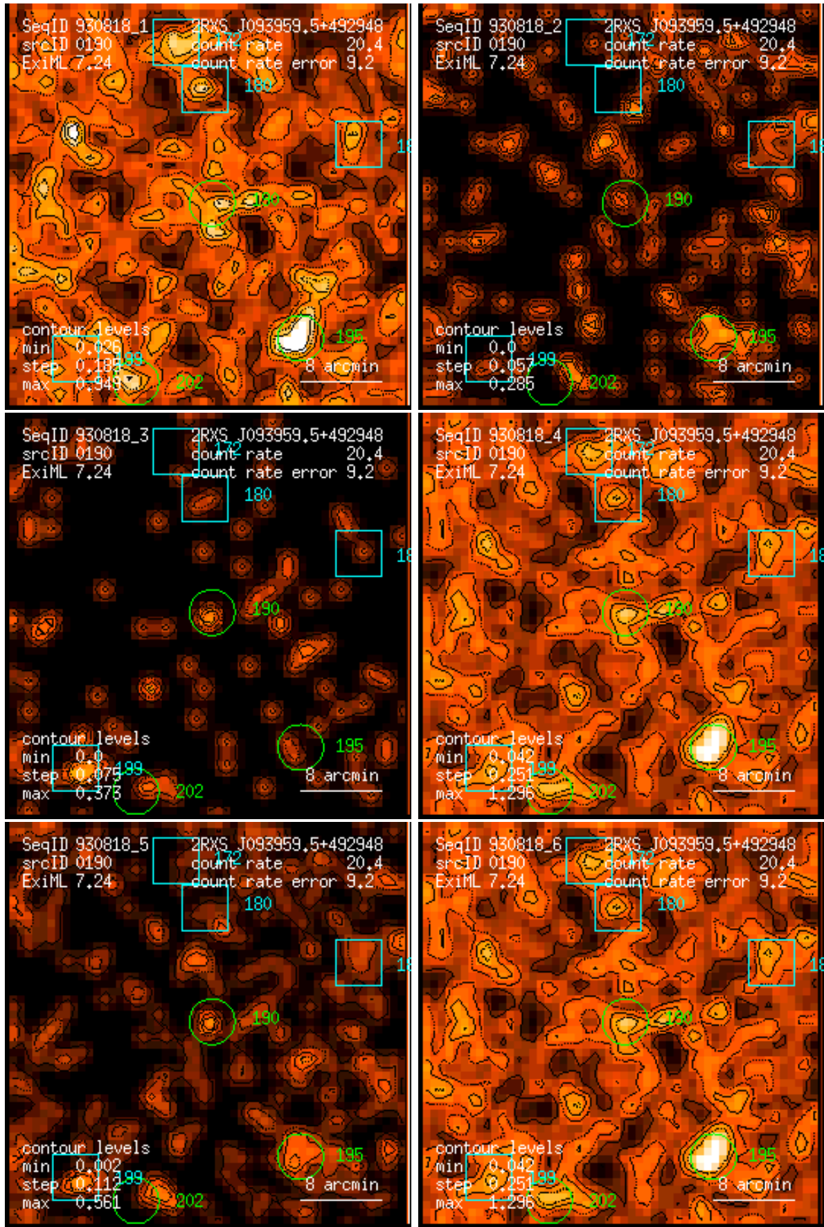
Figure 190: RASS 930818: detection 0190: band rate images, Gaussian filter: (1) PSPC channels 11 – 41, (2) 52 – 90, (3) 91 – 201, (4) 11 – 235, (5) 52 – 201, (6) 11 – 201. Broad band rates in counts/ks. Band rate contour levels in counts/ks/arcmin 2 .
