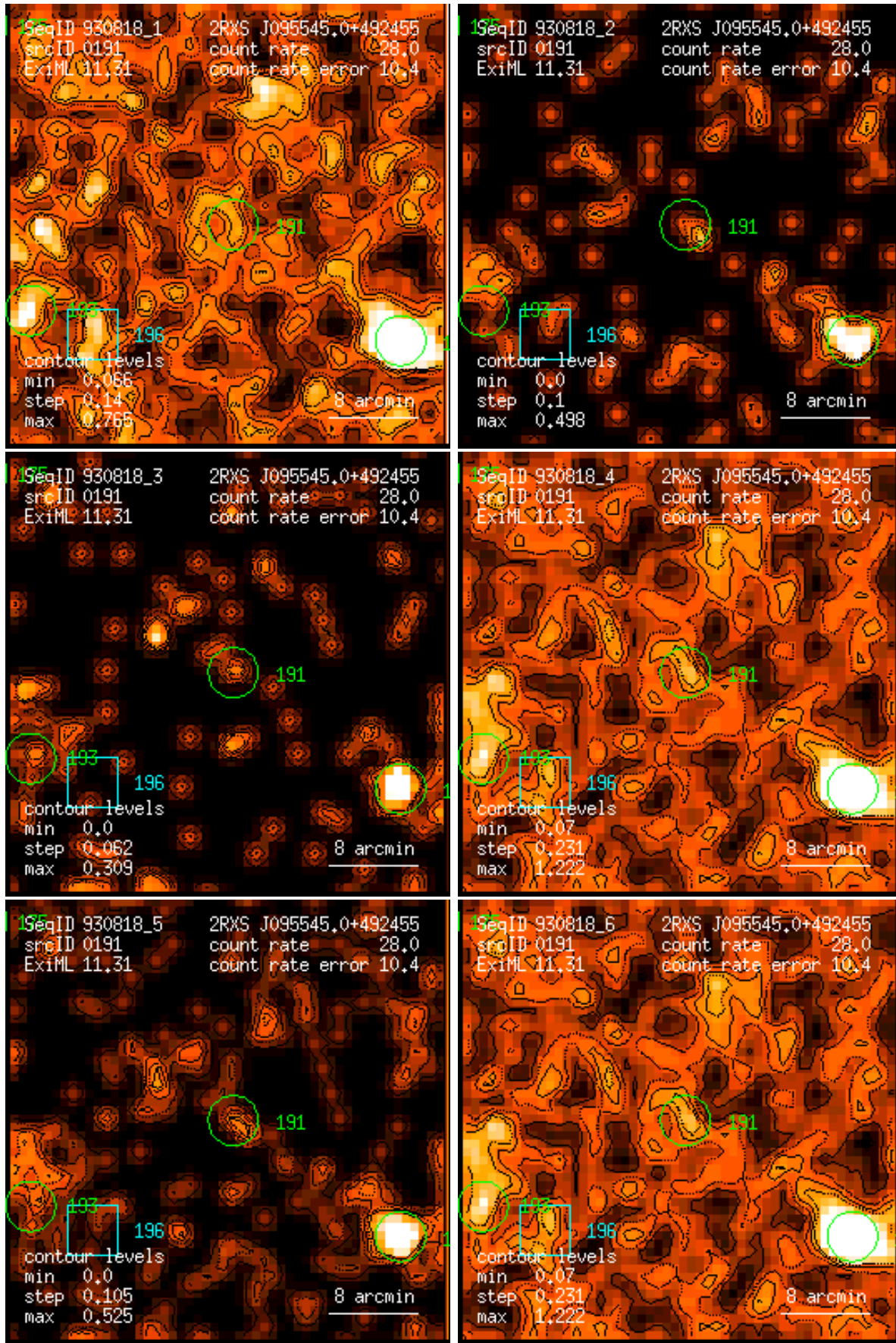
Figure 191: RASS 930818: detection 0191: band rate images, Gaussian filter: (1) PSPC channels 11 – 41, (2) 52 – 90, (3) 91 – 201, (4) 11 – 235, (5) 52 – 201, (6) 11 – 201. Broad band rates in counts/ks. Band rate contour levels in counts/ks/arcmin 2 .
