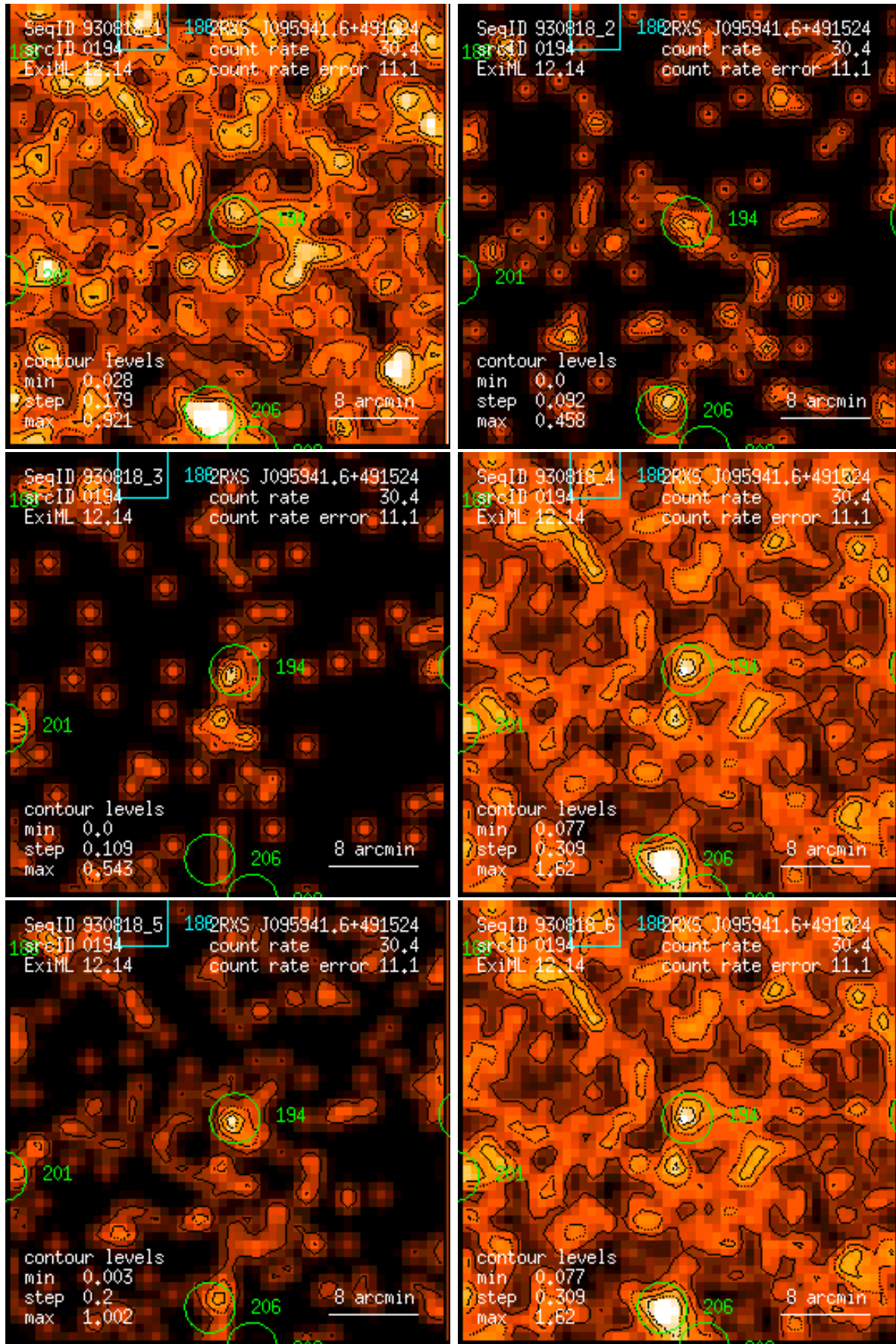
Figure 194: RASS 930818: detection 0194: band rate images, Gaussian filter: (1) PSPC channels 11 – 41, (2) 52 – 90, (3) 91 – 201, (4) 11 – 235, (5) 52 – 201, (6) 11 – 201. Broad band rates in counts/ks. Band rate contour levels in counts/ks/arcmin 2 .
