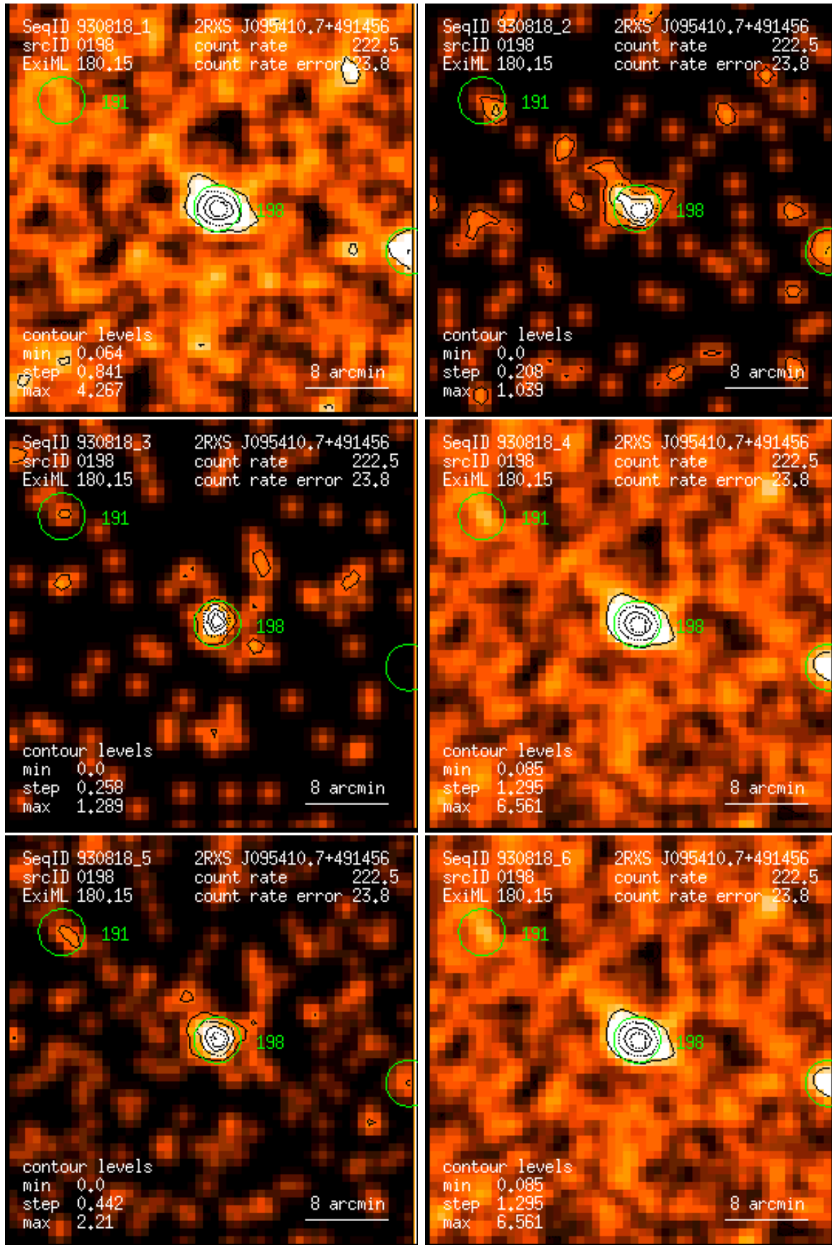
Figure 198: RASS 930818: detection 0198: band rate images, Gaussian filter: (1) PSPC channels 11 – 41, (2) 52 – 90, (3) 91 – 201, (4) 11 – 235, (5) 52 – 201, (6) 11 – 201. Broad band rates in counts/ks. Band rate contour levels in counts/ks/arcmin 2 .
