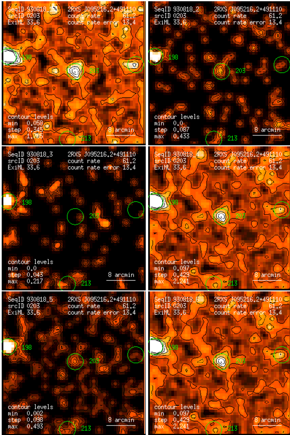
Figure 203: RASS 930818: detection 0203: band rate images, Gaussian filter: (1) PSPC channels 11 – 41, (2) 52 – 90, (3) 91 – 201, (4) 11 – 235, (5) 52 – 201, (6) 11 – 201. Broad band rates in counts/ks. Band rate contour levels in counts/ks/arcmin 2 .
