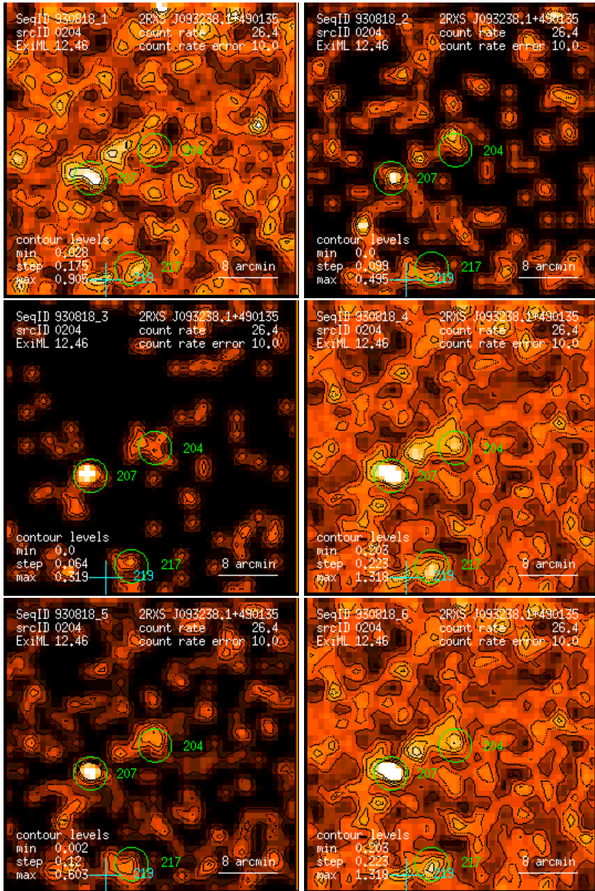
Figure 204: RASS 930818: detection 0204: band rate images, Gaussian filter: (1) PSPC channels 11 – 41, (2) 52 – 90, (3) 91 – 201, (4) 11 – 235, (5) 52 – 201, (6) 11 – 201. Broad band rates in counts/ks. Band rate contour levels in counts/ks/arcmin 2 .
