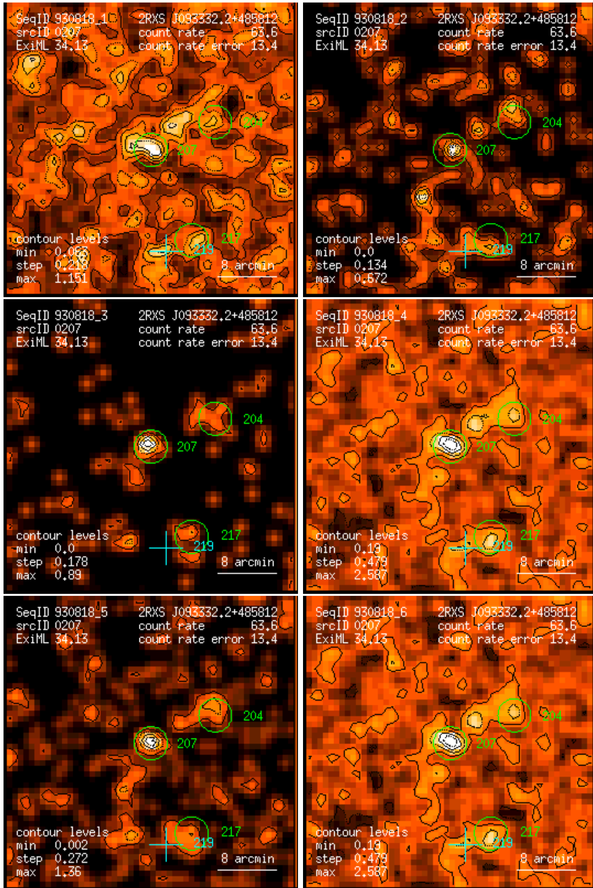
Figure 207: RASS 930818: detection 0207: band rate images, Gaussian filter: (1) PSPC channels 11 – 41, (2) 52 – 90, (3) 91 – 201, (4) 11 – 235, (5) 52 – 201, (6) 11 – 201. Broad band rates in counts/ks. Band rate contour levels in counts/ks/arcmin 2 .
