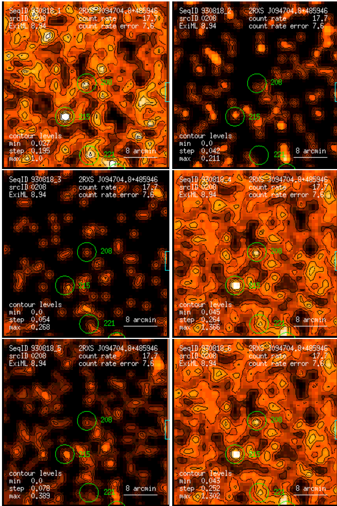
Figure 208: RASS 930818: detection 0208: band rate images, Gaussian filter: (1) PSPC channels 11 – 41, (2) 52 – 90, (3) 91 – 201, (4) 11 – 235, (5) 52 – 201, (6) 11 – 201. Broad band rates in counts/ks. Band rate contour levels in counts/ks/arcmin 2 .
