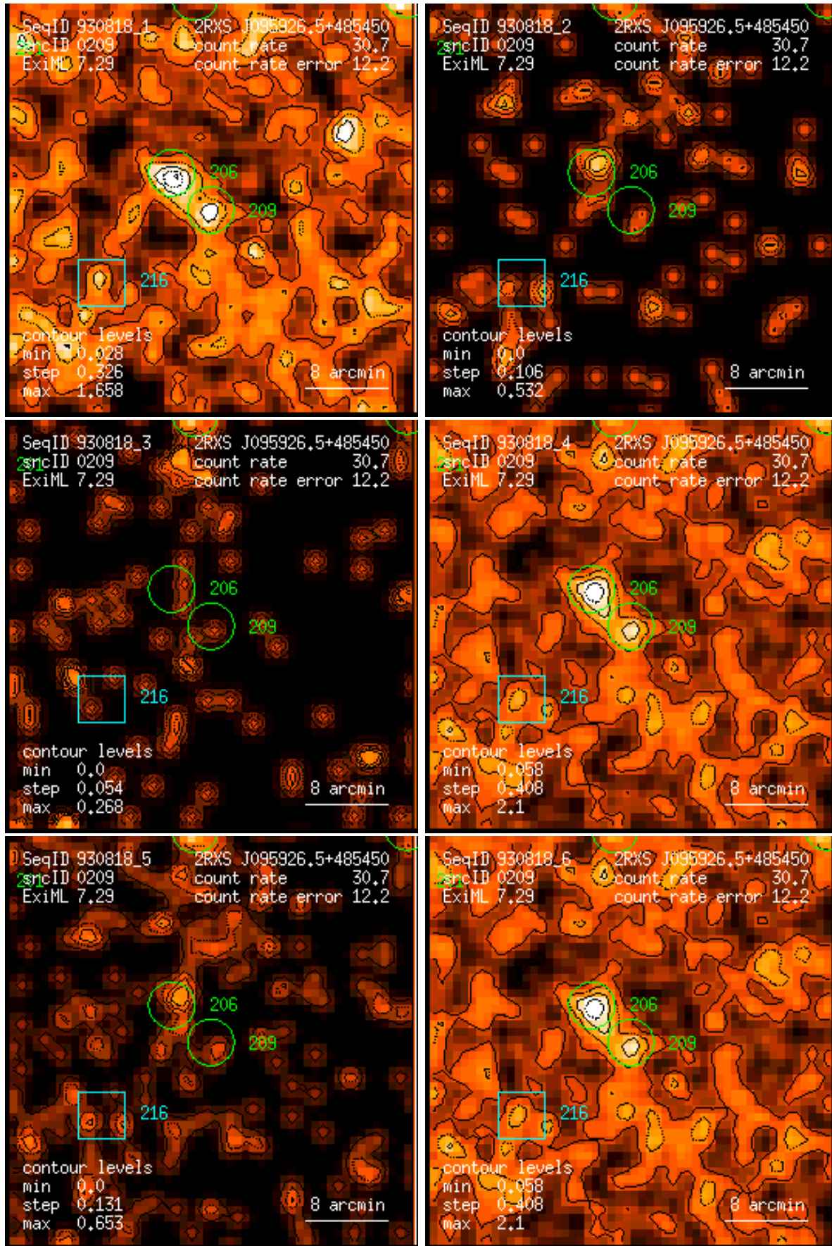
Figure 209: RASS 930818: detection 0209: band rate images, Gaussian filter: (1) PSPC channels 11 – 41, (2) 52 – 90, (3) 91 – 201, (4) 11 – 235, (5) 52 – 201, (6) 11 – 201. Broad band rates in counts/ks. Band rate contour levels in counts/ks/arcmin 2 .
