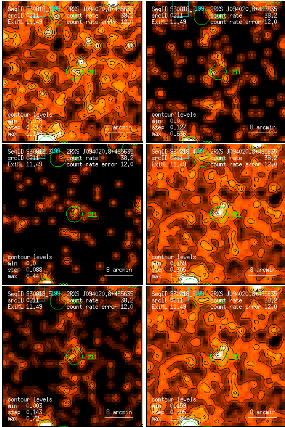
Figure 211: RASS 930818: detection 0211: band rate images, Gaussian filter: (1) PSPC channels 11 – 41, (2) 52 – 90, (3) 91 – 201, (4) 11 – 235, (5) 52 – 201, (6) 11 – 201. Broad band rates in counts/ks. Band rate contour levels in counts/ks/arcmin 2 .
