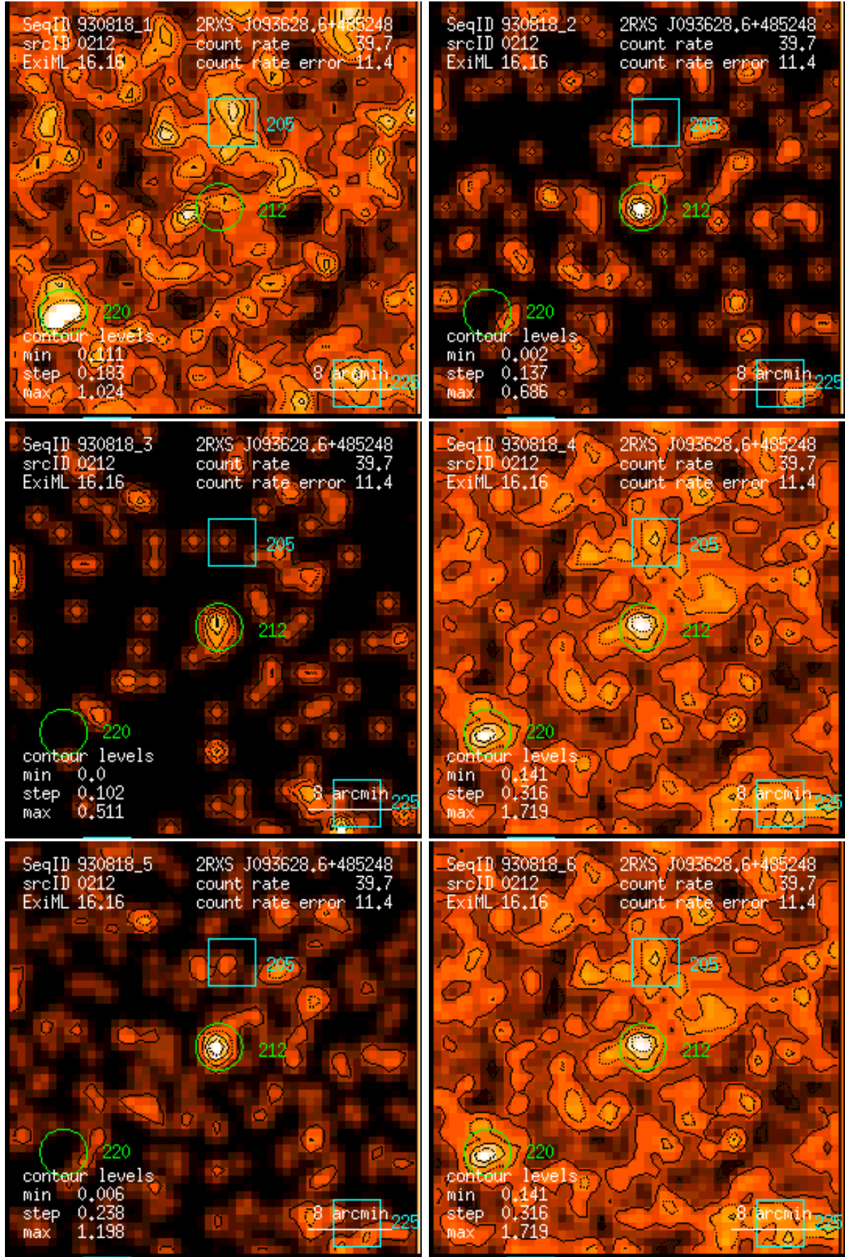
Figure 212: RASS 930818: detection 0212: band rate images, Gaussian filter: (1) PSPC channels 11 – 41, (2) 52 – 90, (3) 91 – 201, (4) 11 – 235, (5) 52 – 201, (6) 11 – 201. Broad band rates in counts/ks. Band rate contour levels in counts/ks/arcmin 2 .
