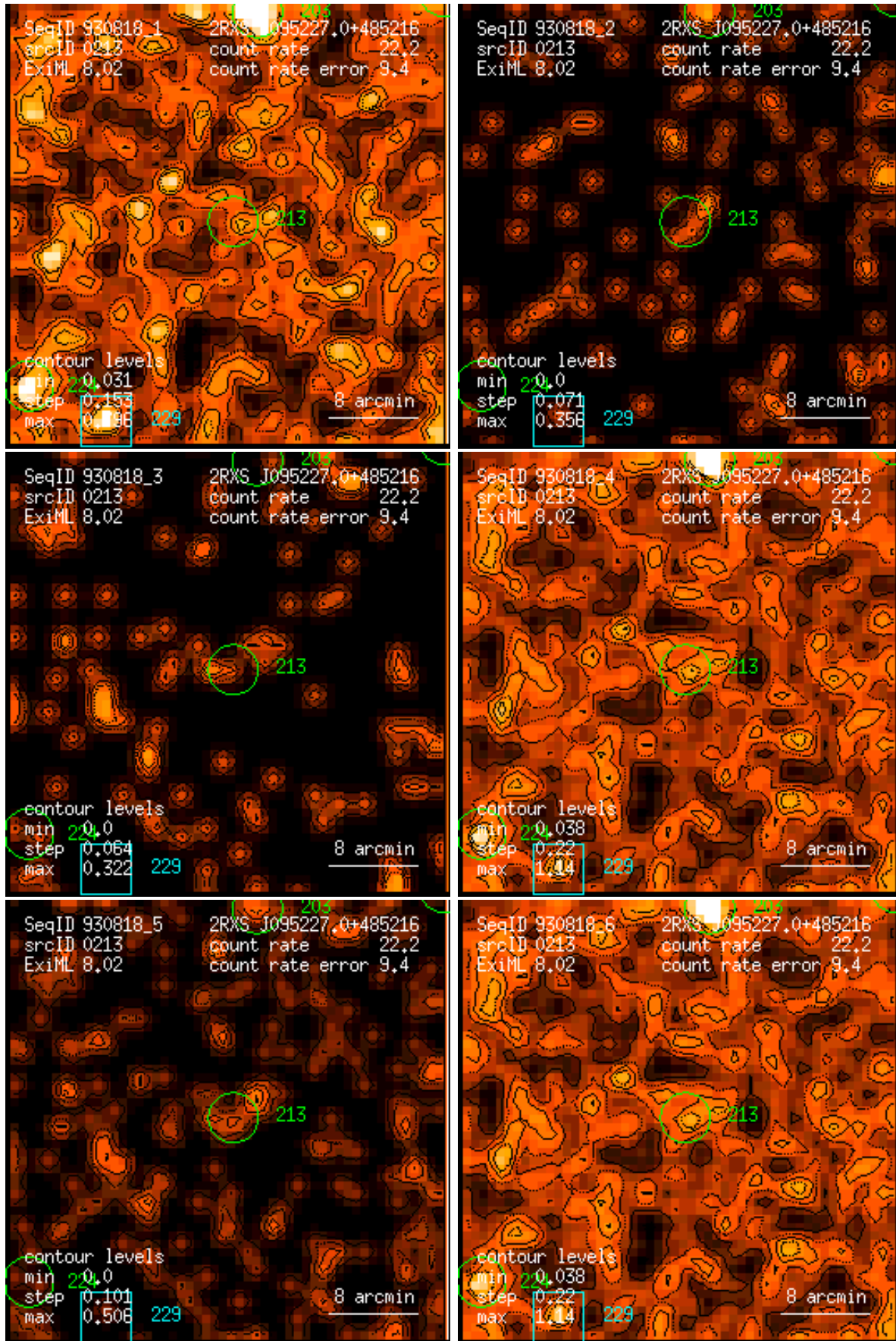
Figure 213: RASS 930818: detection 0213: band rate images, Gaussian filter: (1) PSPC channels 11 – 41, (2) 52 – 90, (3) 91 – 201, (4) 11 – 235, (5) 52 – 201, (6) 11 – 201. Broad band rates in counts/ks. Band rate contour levels in counts/ks/arcmin 2 .
