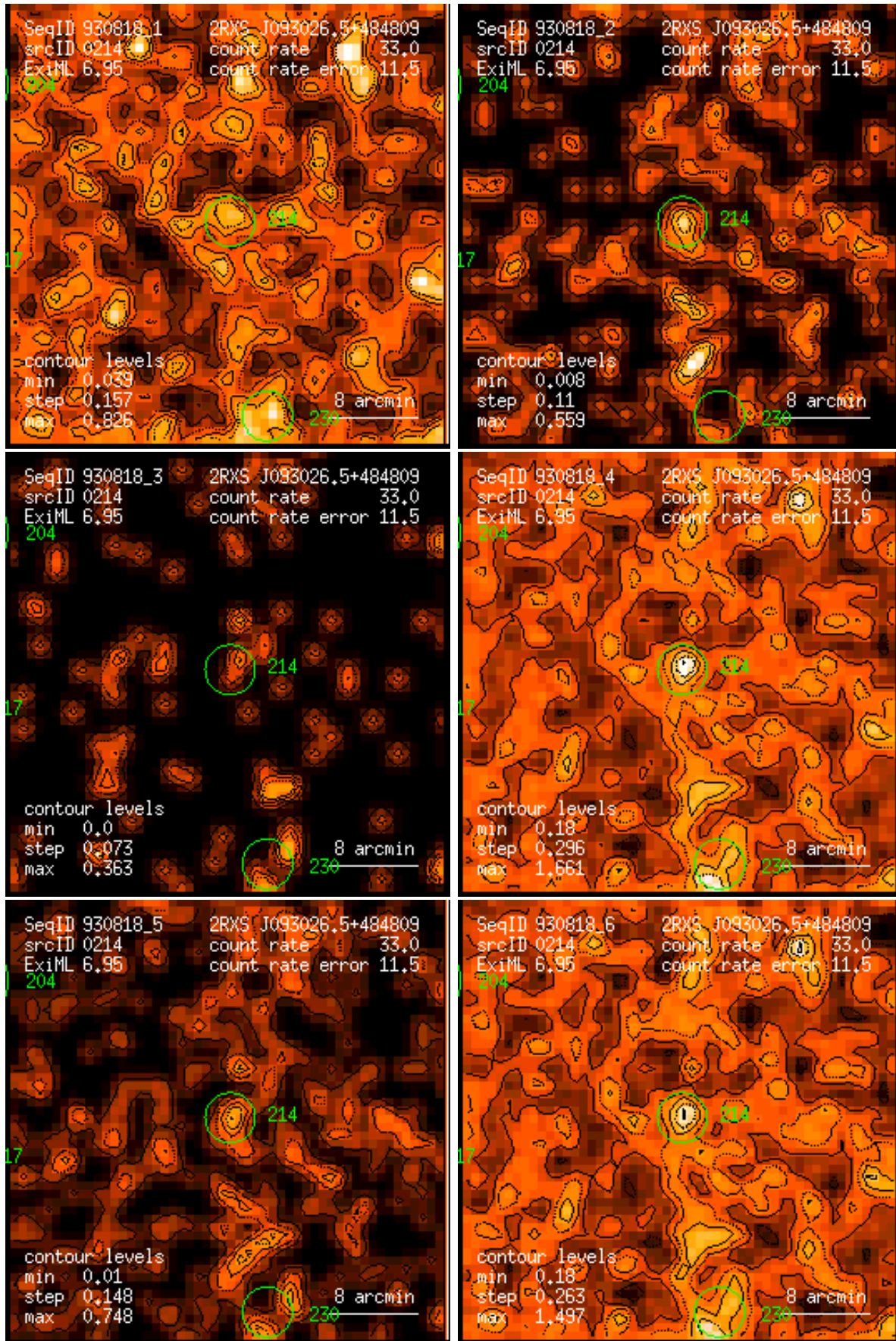
Figure 214: RASS 930818: detection 0214: band rate images, Gaussian filter: (1) PSPC channels 11 – 41, (2) 52 – 90, (3) 91 – 201, (4) 11 – 235, (5) 52 – 201, (6) 11 – 201. Broad band rates in counts/ks. Band rate contour levels in counts/ks/arcmin 2 .
