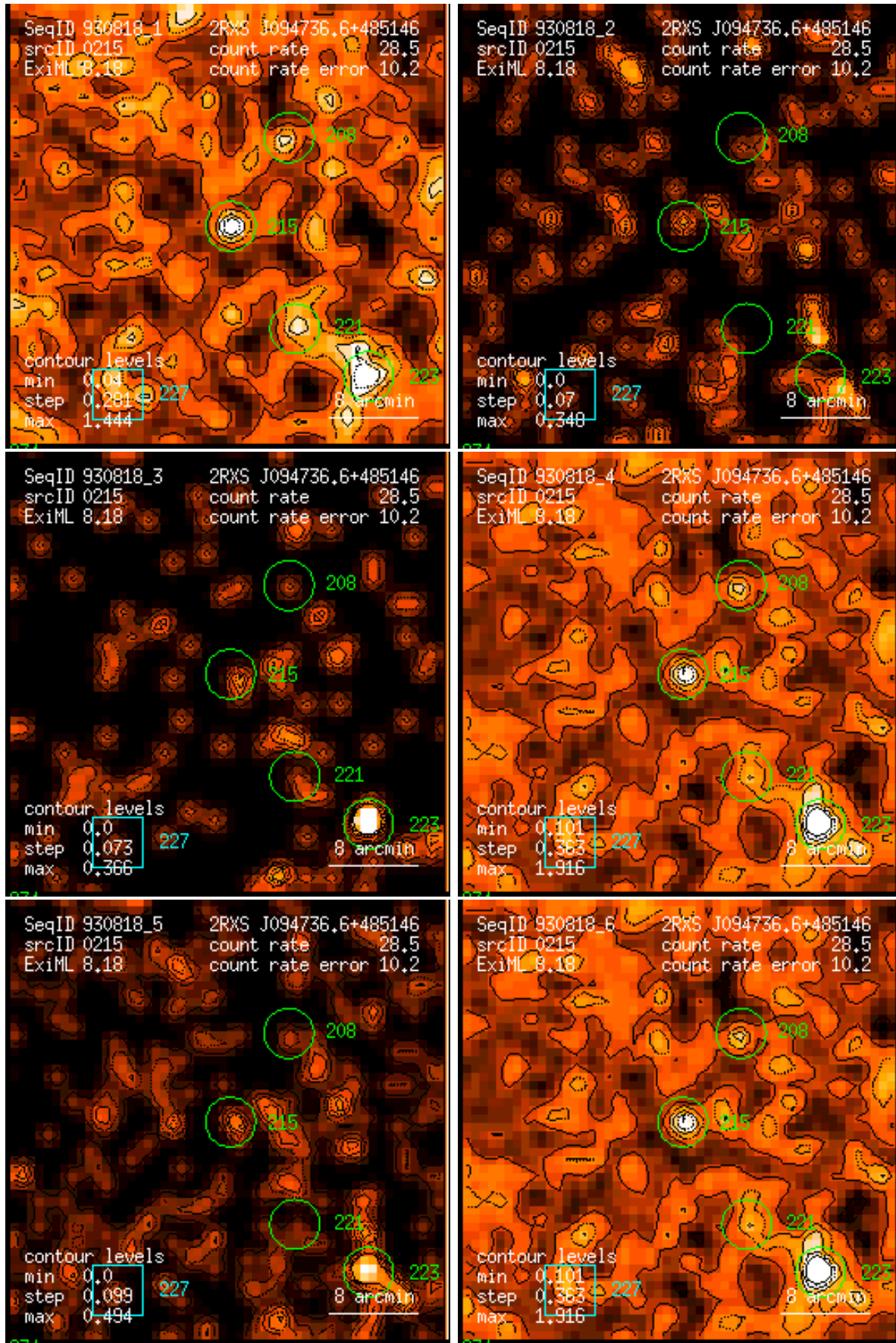
Figure 215: RASS 930818: detection 0215: band rate images, Gaussian filter: (1) PSPC channels 11 – 41, (2) 52 – 90, (3) 91 – 201, (4) 11 – 235, (5) 52 – 201, (6) 11 – 201. Broad band rates in counts/ks. Band rate contour levels in counts/ks/arcmin 2 .
