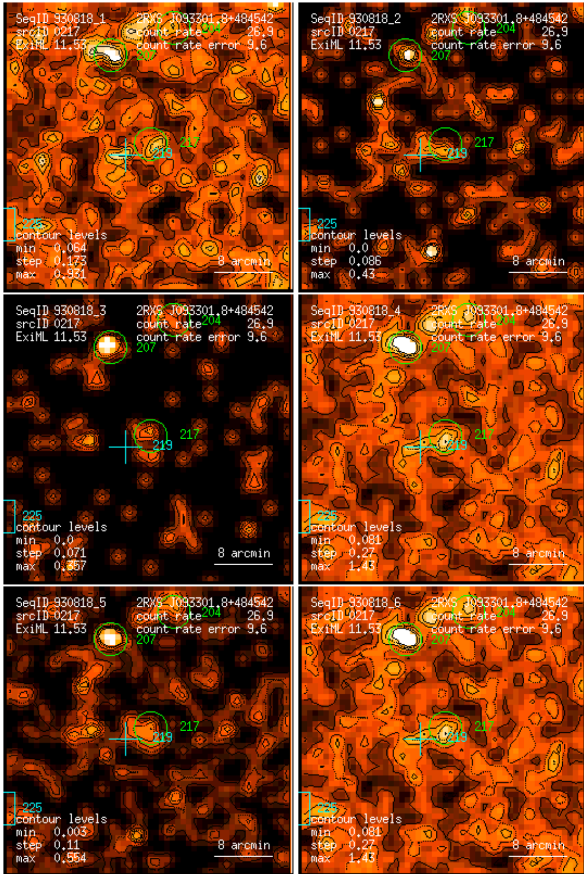
Figure 217: RASS 930818: detection 0217: band rate images, Gaussian filter: (1) PSPC channels 11 – 41, (2) 52 – 90, (3) 91 – 201, (4) 11 – 235, (5) 52 – 201, (6) 11 – 201. Broad band rates in counts/ks. Band rate contour levels in counts/ks/arcmin 2 .
