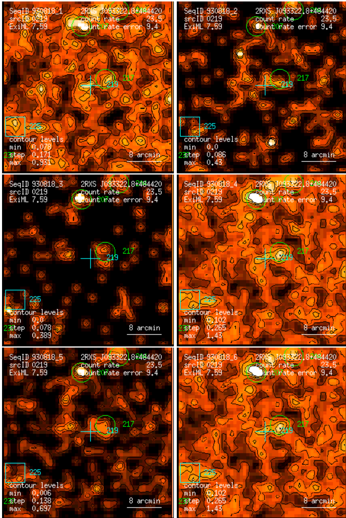
Figure 219: RASS 930818: detection 0219: band rate images, Gaussian filter: (1) PSPC channels 11 – 41, (2) 52 – 90, (3) 91 – 201, (4) 11 – 235, (5) 52 – 201, (6) 11 – 201. Broad band rates in counts/ks. Band rate contour levels in counts/ks/arcmin 2 .
