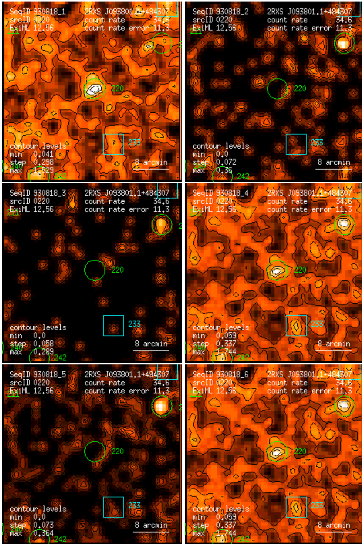
Figure 220: RASS 930818: detection 0220: band rate images, Gaussian filter: (1) PSPC channels 11 – 41, (2) 52 – 90, (3) 91 – 201, (4) 11 – 235, (5) 52 – 201, (6) 11 – 201. Broad band rates in counts/ks. Band rate contour levels in counts/ks/arcmin 2 .
