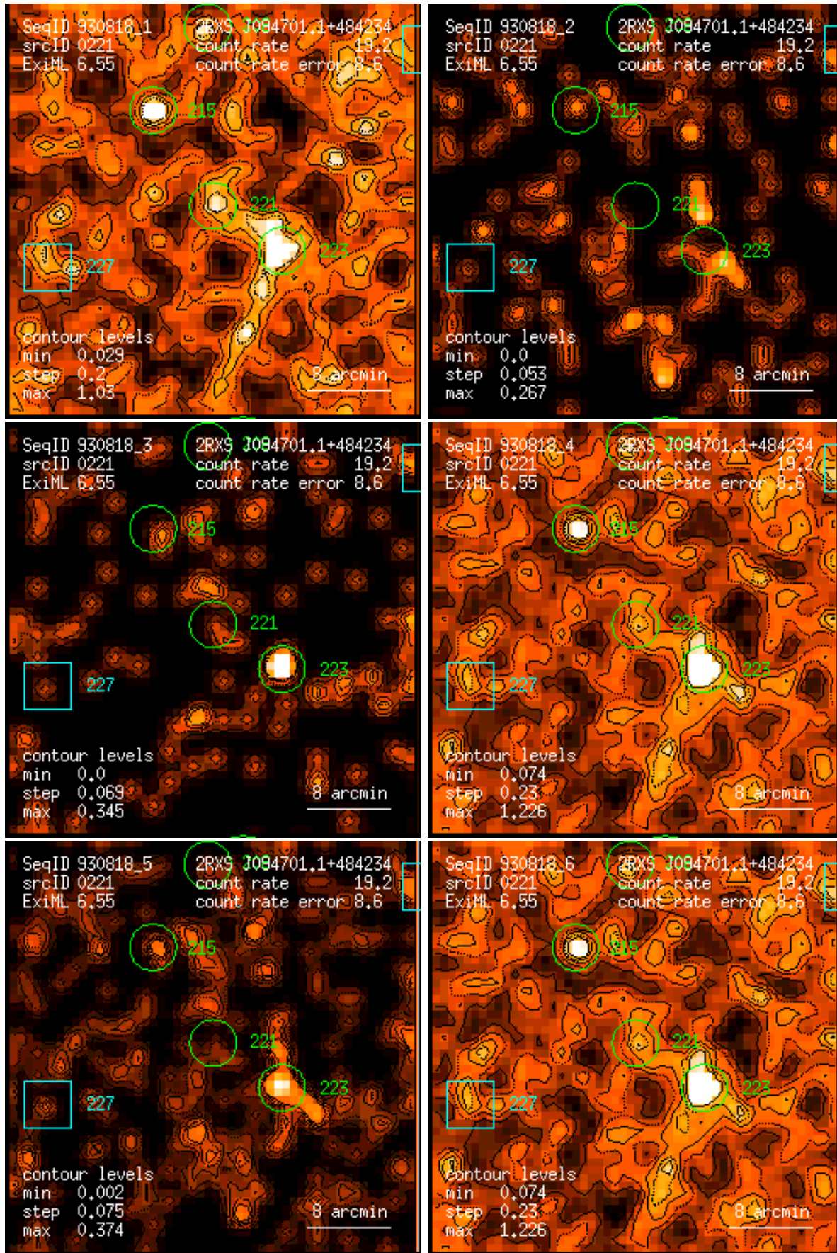
Figure 221: RASS 930818: detection 0221: band rate images, Gaussian filter: (1) PSPC channels 11 – 41, (2) 52 – 90, (3) 91 – 201, (4) 11 – 235, (5) 52 – 201, (6) 11 – 201. Broad band rates in counts/ks. Band rate contour levels in counts/ks/arcmin 2 .
