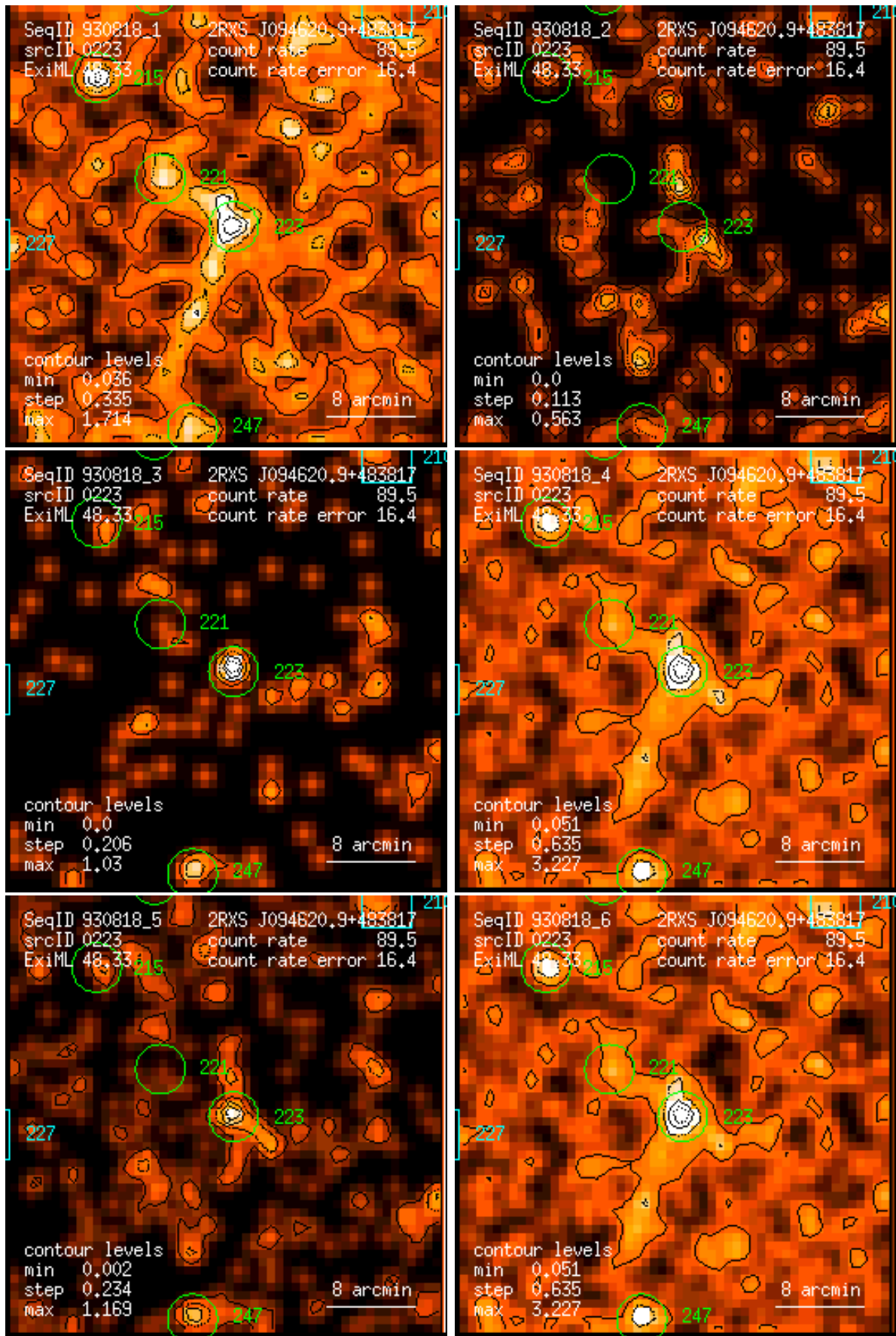
Figure 223: RASS 930818: detection 0223: band rate images, Gaussian filter: (1) PSPC channels 11 – 41, (2) 52 – 90, (3) 91 – 201, (4) 11 – 235, (5) 52 – 201, (6) 11 – 201. Broad band rates in counts/ks. Band rate contour levels in counts/ks/arcmin 2 .
