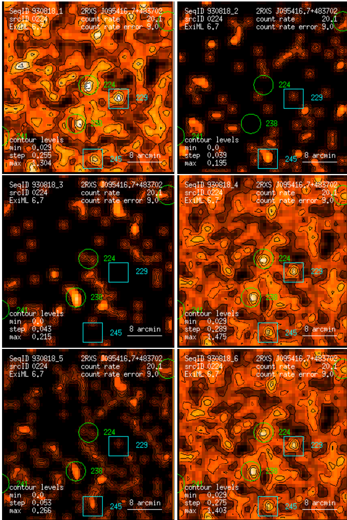
Figure 224: RASS 930818: detection 0224: band rate images, Gaussian filter: (1) PSPC channels 11 – 41, (2) 52 – 90, (3) 91 – 201, (4) 11 – 235, (5) 52 – 201, (6) 11 – 201. Broad band rates in counts/ks. Band rate contour levels in counts/ks/arcmin 2 .
