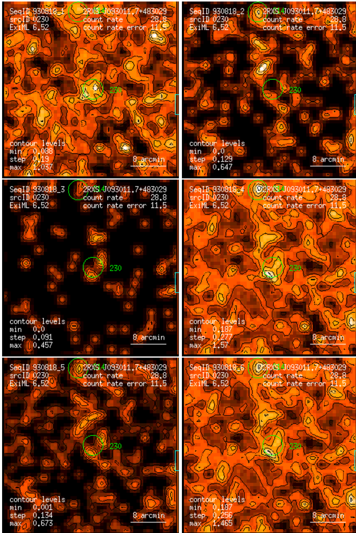
Figure 230: RASS 930818: detection 0230: band rate images, Gaussian filter: (1) PSPC channels 11 – 41, (2) 52 – 90, (3) 91 – 201, (4) 11 – 235, (5) 52 – 201, (6) 11 – 201. Broad band rates in counts/ks. Band rate contour levels in counts/ks/arcmin 2 .
