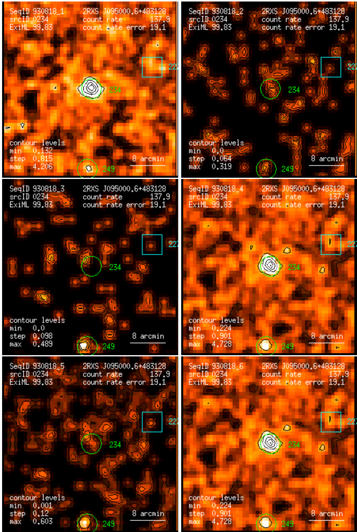
Figure 234: RASS 930818: detection 0234: band rate images, Gaussian filter: (1) PSPC channels 11 – 41, (2) 52 – 90, (3) 91 – 201, (4) 11 – 235, (5) 52 – 201, (6) 11 – 201. Broad band rates in counts/ks. Band rate contour levels in counts/ks/arcmin 2 .
