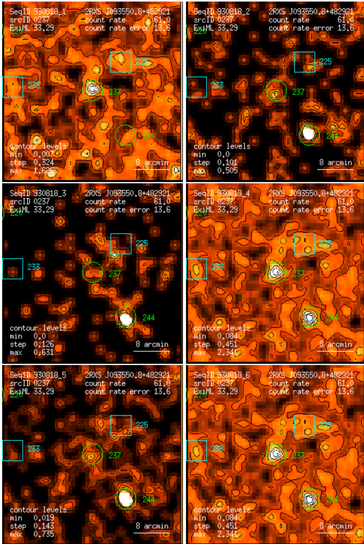
Figure 237: RASS 930818: detection 0237: band rate images, Gaussian filter: (1) PSPC channels 11 – 41, (2) 52 – 90, (3) 91 – 201, (4) 11 – 235, (5) 52 – 201, (6) 11 – 201. Broad band rates in counts/ks. Band rate contour levels in counts/ks/arcmin 2 .
