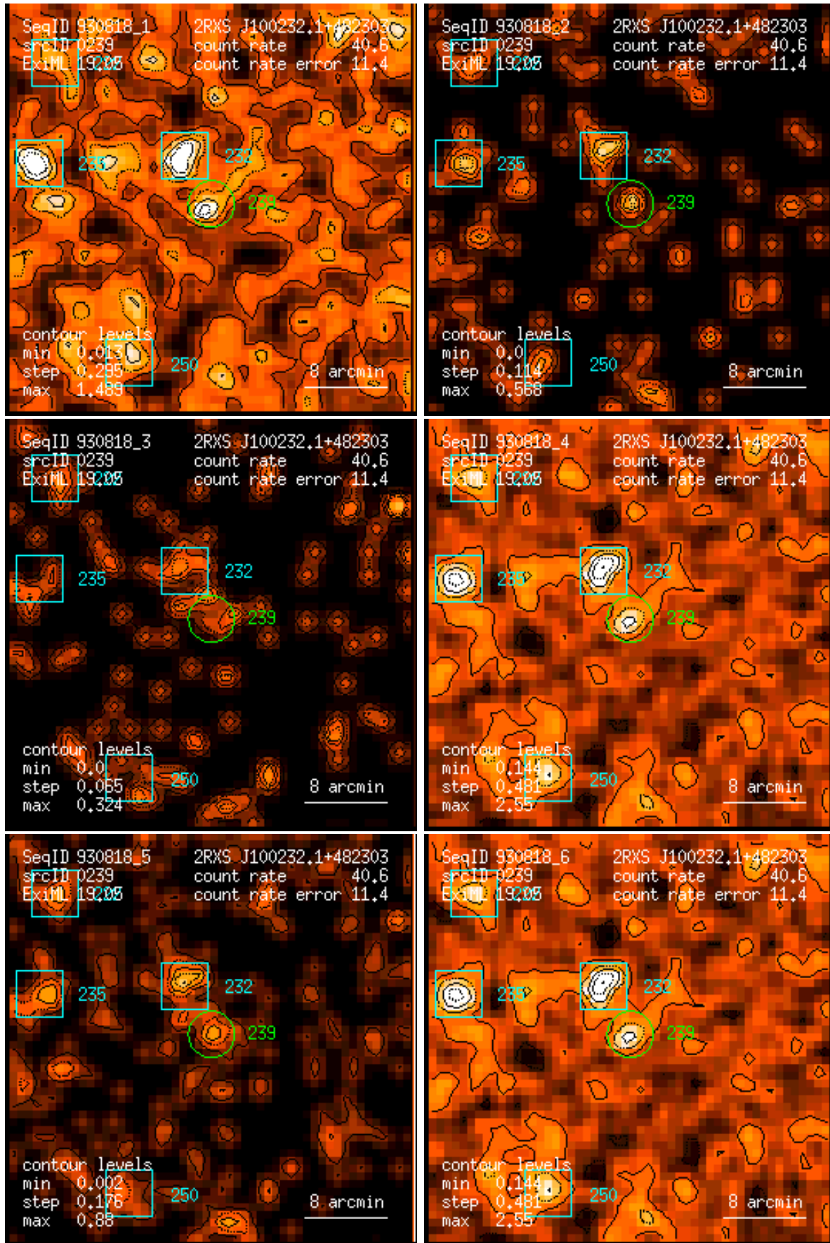
Figure 239: RASS 930818: detection 0239: band rate images, Gaussian filter: (1) PSPC channels 11 – 41, (2) 52 – 90, (3) 91 – 201, (4) 11 – 235, (5) 52 – 201, (6) 11 – 201. Broad band rates in counts/ks. Band rate contour levels in counts/ks/arcmin 2 .
