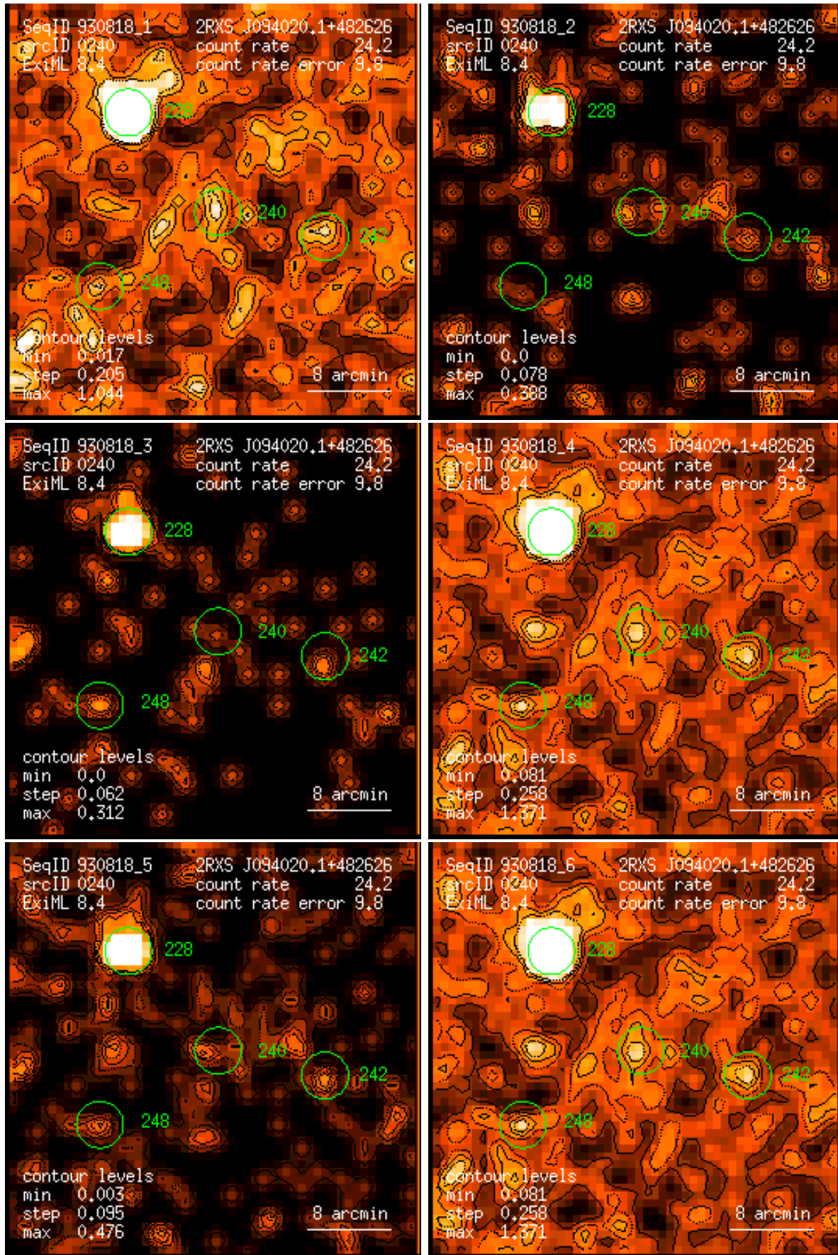
Figure 240: RASS 930818: detection 0240: band rate images, Gaussian filter: (1) PSPC channels 11 – 41, (2) 52 – 90, (3) 91 – 201, (4) 11 – 235, (5) 52 – 201, (6) 11 – 201. Broad band rates in counts/ks. Band rate contour levels in counts/ks/arcmin 2 .
