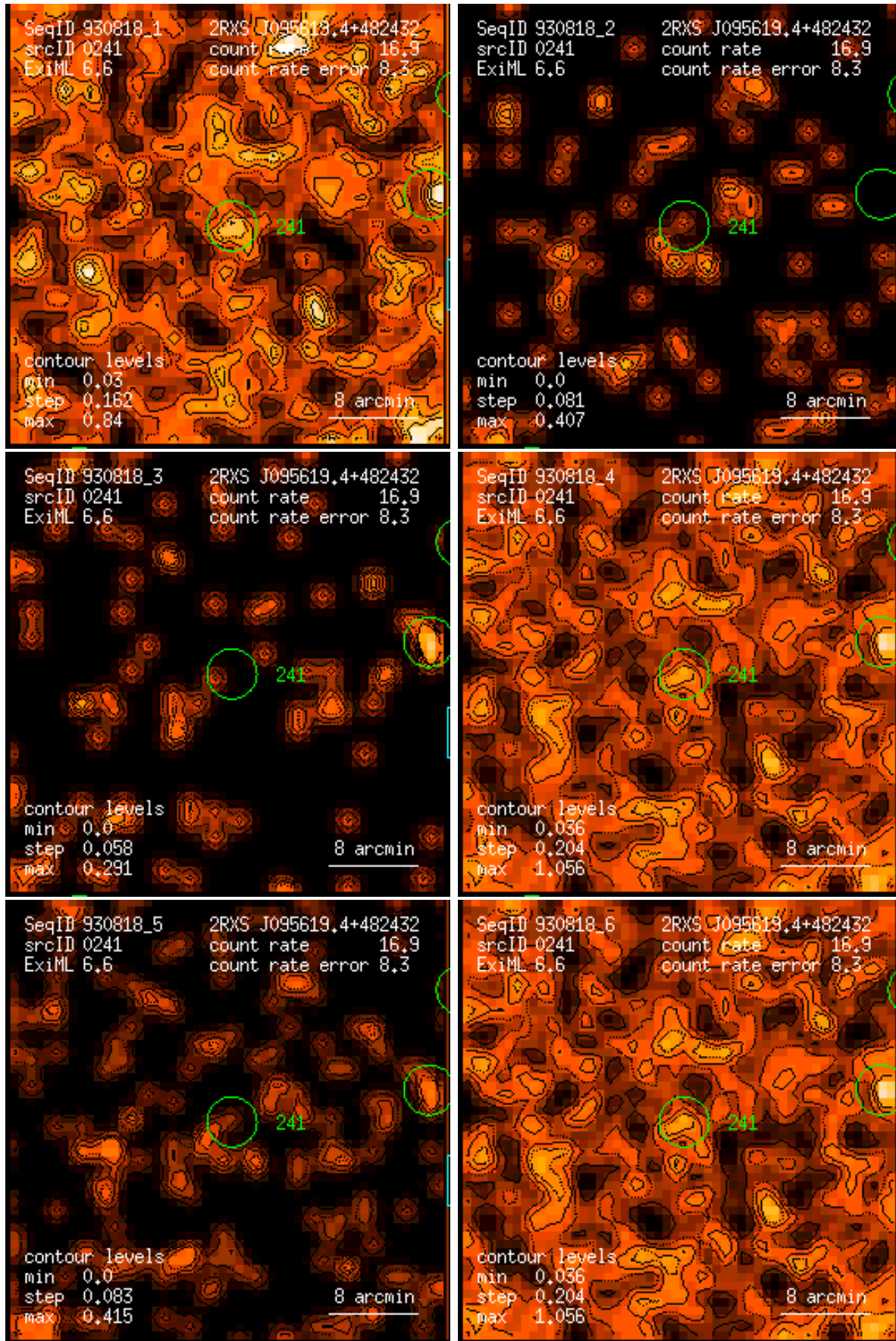
Figure 241: RASS 930818: detection 0241: band rate images, Gaussian filter: (1) PSPC channels 11 – 41, (2) 52 – 90, (3) 91 – 201, (4) 11 – 235, (5) 52 – 201, (6) 11 – 201. Broad band rates in counts/ks. Band rate contour levels in counts/ks/arcmin 2 .
