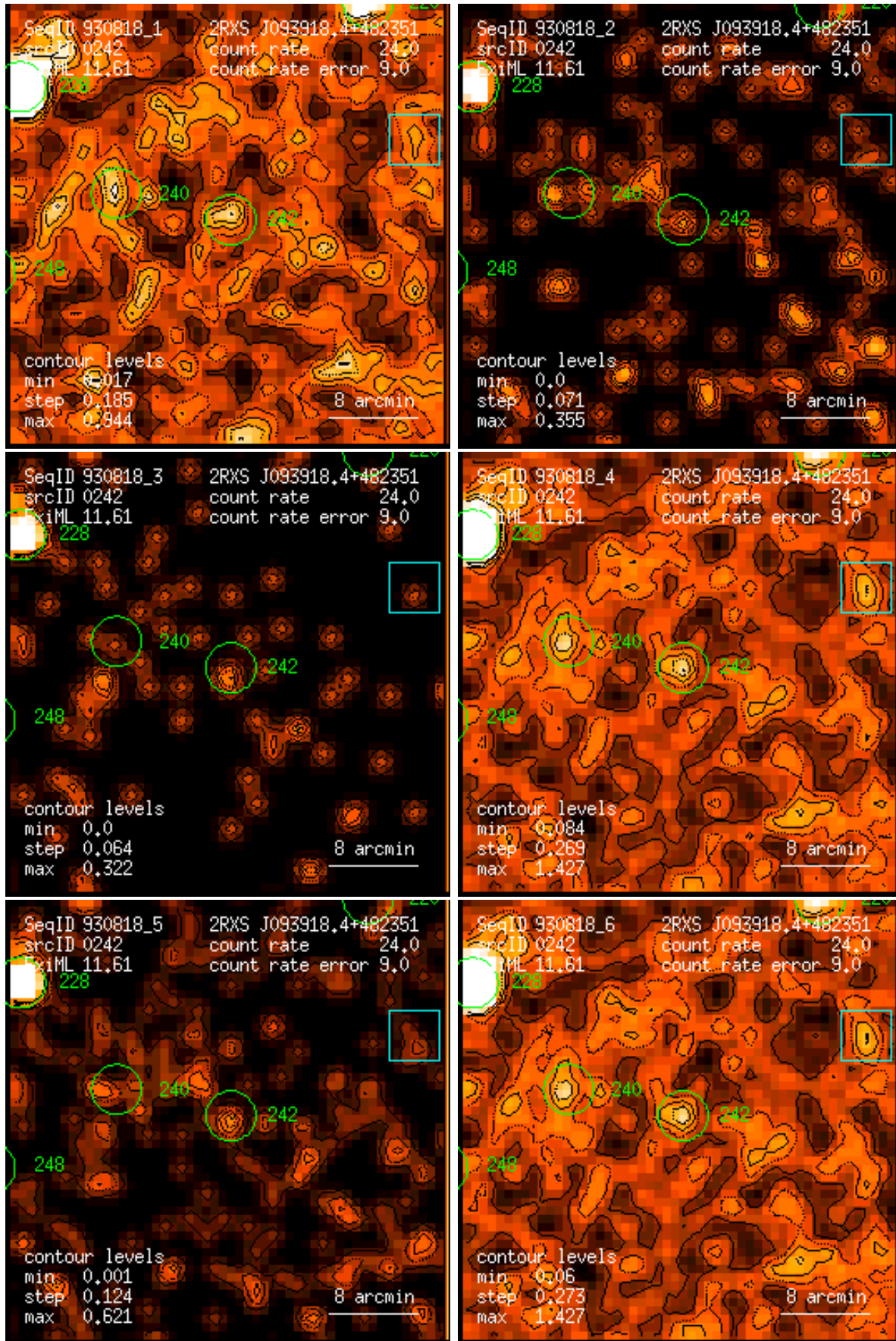
Figure 242: RASS 930818: detection 0242: band rate images, Gaussian filter: (1) PSPC channels 11 – 41, (2) 52 – 90, (3) 91 – 201, (4) 11 – 235, (5) 52 – 201, (6) 11 – 201. Broad band rates in counts/ks. Band rate contour levels in counts/ks/arcmin 2 .
