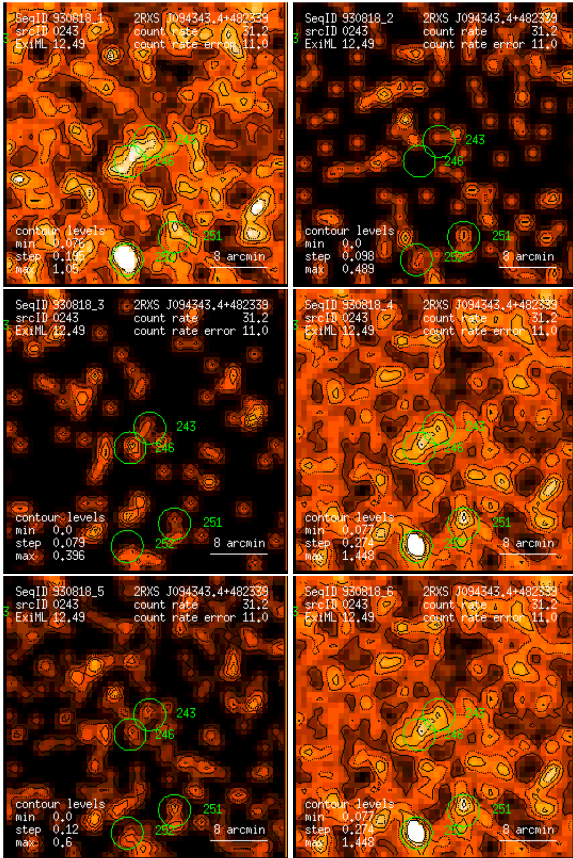
Figure 243: RASS 930818: detection 0243: band rate images, Gaussian filter: (1) PSPC channels 11 – 41, (2) 52 – 90, (3) 91 – 201, (4) 11 – 235, (5) 52 – 201, (6) 11 – 201. Broad band rates in counts/ks. Band rate contour levels in counts/ks/arcmin 2 .
