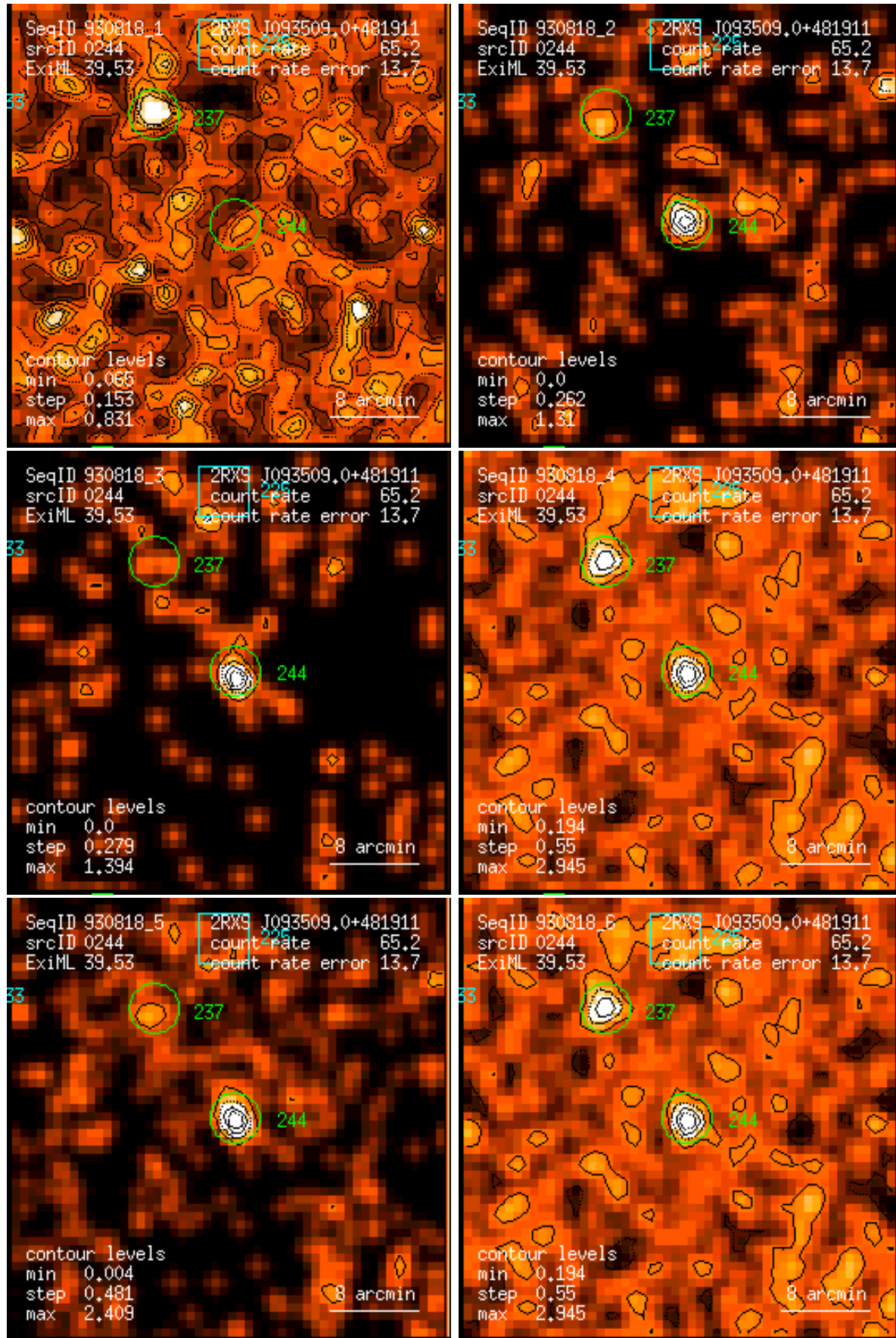
Figure 244: RASS 930818: detection 0244: band rate images, Gaussian filter: (1) PSPC channels 11 – 41, (2) 52 – 90, (3) 91 – 201, (4) 11 – 235, (5) 52 – 201, (6) 11 – 201. Broad band rates in counts/ks. Band rate contour levels in counts/ks/arcmin 2 .
