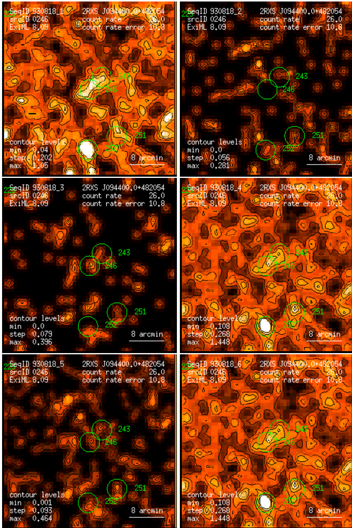
Figure 246: RASS 930818: detection 0246: band rate images, Gaussian filter: (1) PSPC channels 11 – 41, (2) 52 – 90, (3) 91 – 201, (4) 11 – 235, (5) 52 – 201, (6) 11 – 201. Broad band rates in counts/ks. Band rate contour levels in counts/ks/arcmin 2 .
