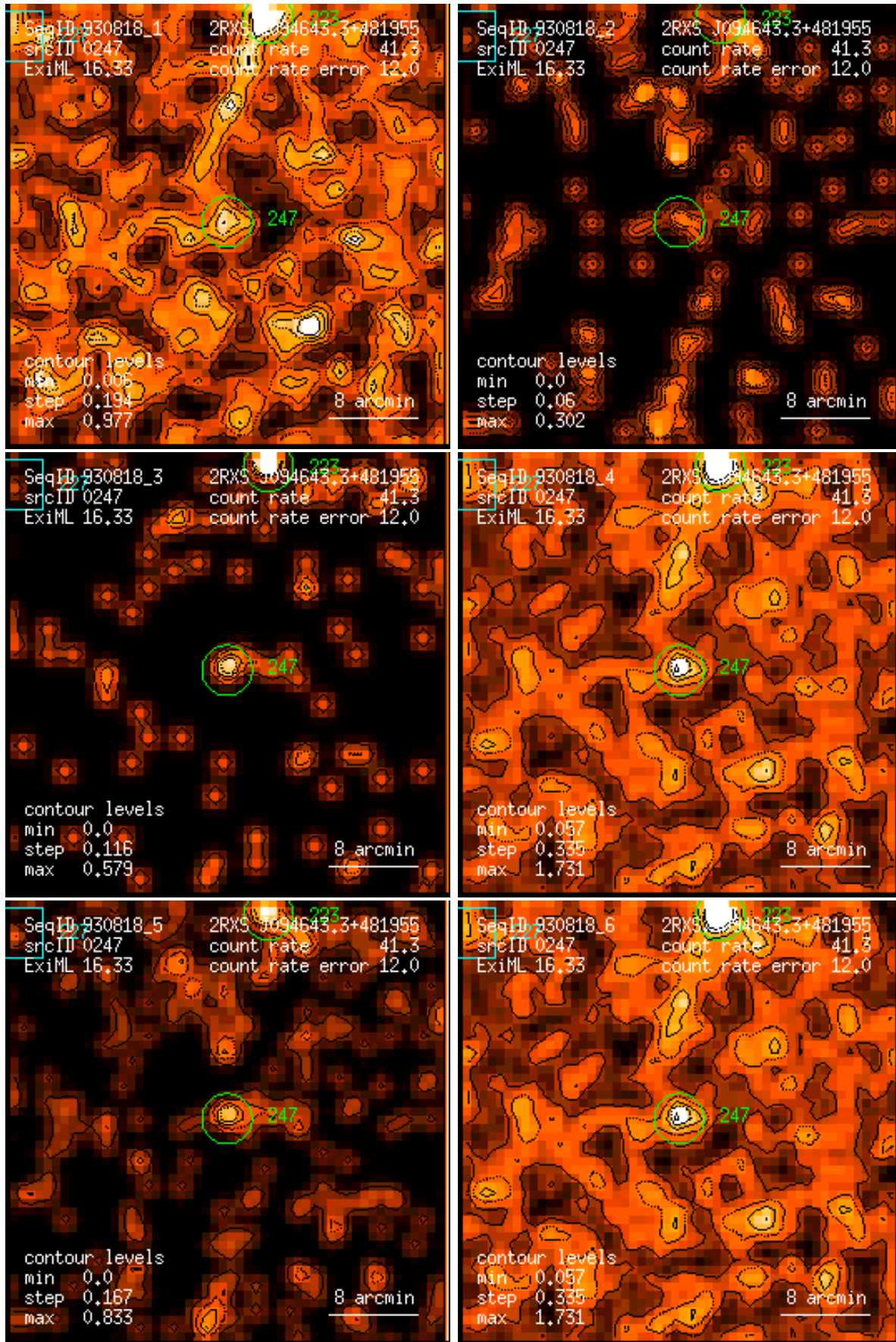
Figure 247: RASS 930818: detection 0247: band rate images, Gaussian filter: (1) PSPC channels 11 – 41, (2) 52 – 90, (3) 91 – 201, (4) 11 – 235, (5) 52 – 201, (6) 11 – 201. Broad band rates in counts/ks. Band rate contour levels in counts/ks/arcmin 2 .
