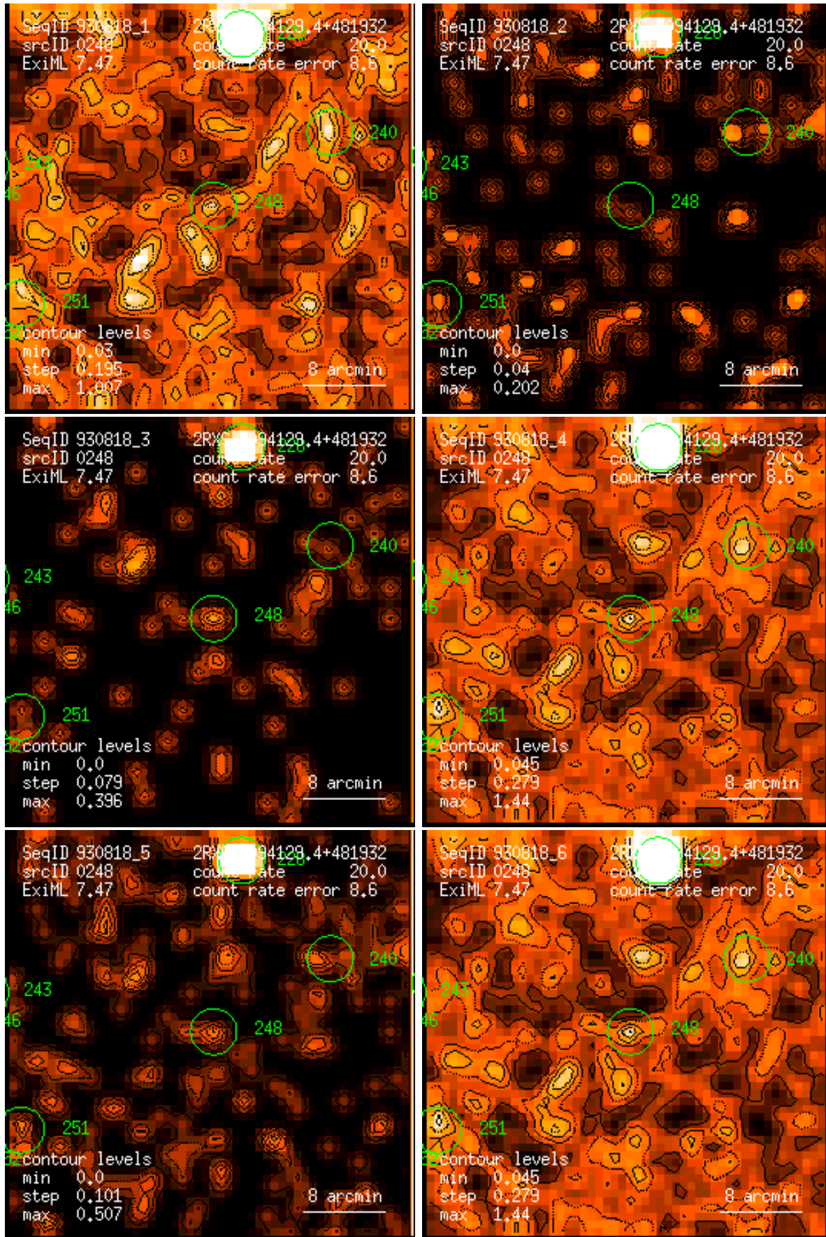
Figure 248: RASS 930818: detection 0248: band rate images, Gaussian filter: (1) PSPC channels 11 – 41, (2) 52 – 90, (3) 91 – 201, (4) 11 – 235, (5) 52 – 201, (6) 11 – 201. Broad band rates in counts/ks. Band rate contour levels in counts/ks/arcmin 2 .
