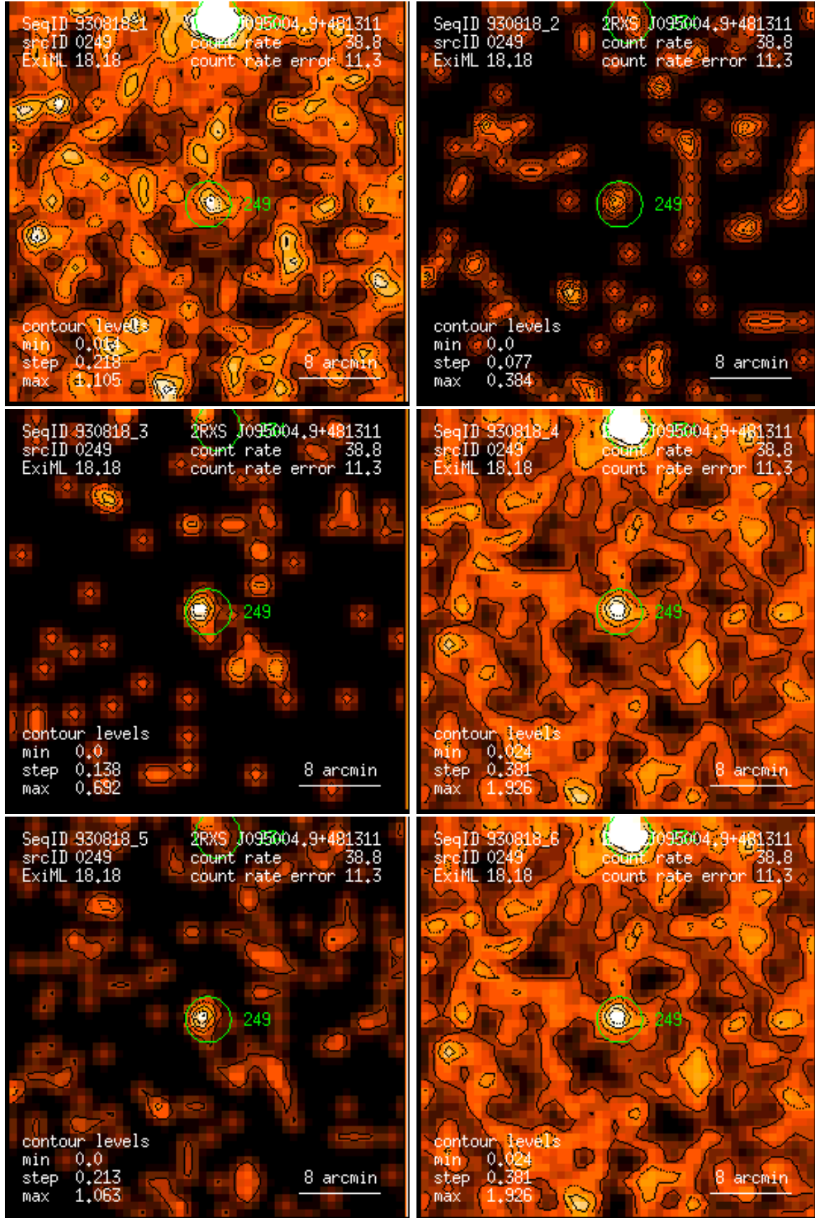
Figure 249: RASS 930818: detection 0249: band rate images, Gaussian filter: (1) PSPC channels 11 – 41, (2) 52 – 90, (3) 91 – 201, (4) 11 – 235, (5) 52 – 201, (6) 11 – 201. Broad band rates in counts/ks. Band rate contour levels in counts/ks/arcmin 2 .
