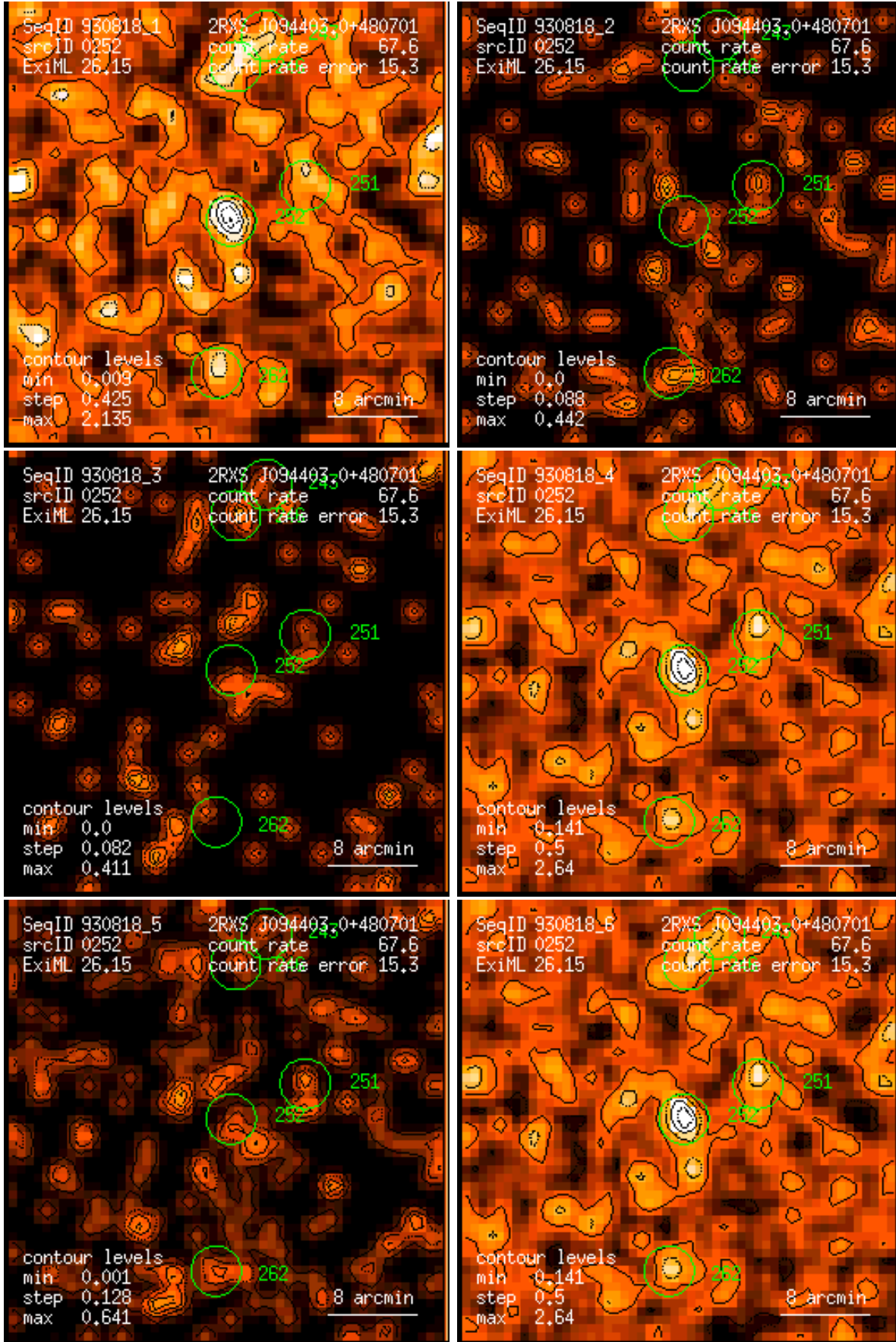
Figure 252: RASS 930818: detection 0252: band rate images, Gaussian filter: (1) PSPC channels 11 – 41, (2) 52 – 90, (3) 91 – 201, (4) 11 – 235, (5) 52 – 201, (6) 11 – 201. Broad band rates in counts/ks. Band rate contour levels in counts/ks/arcmin 2 .
