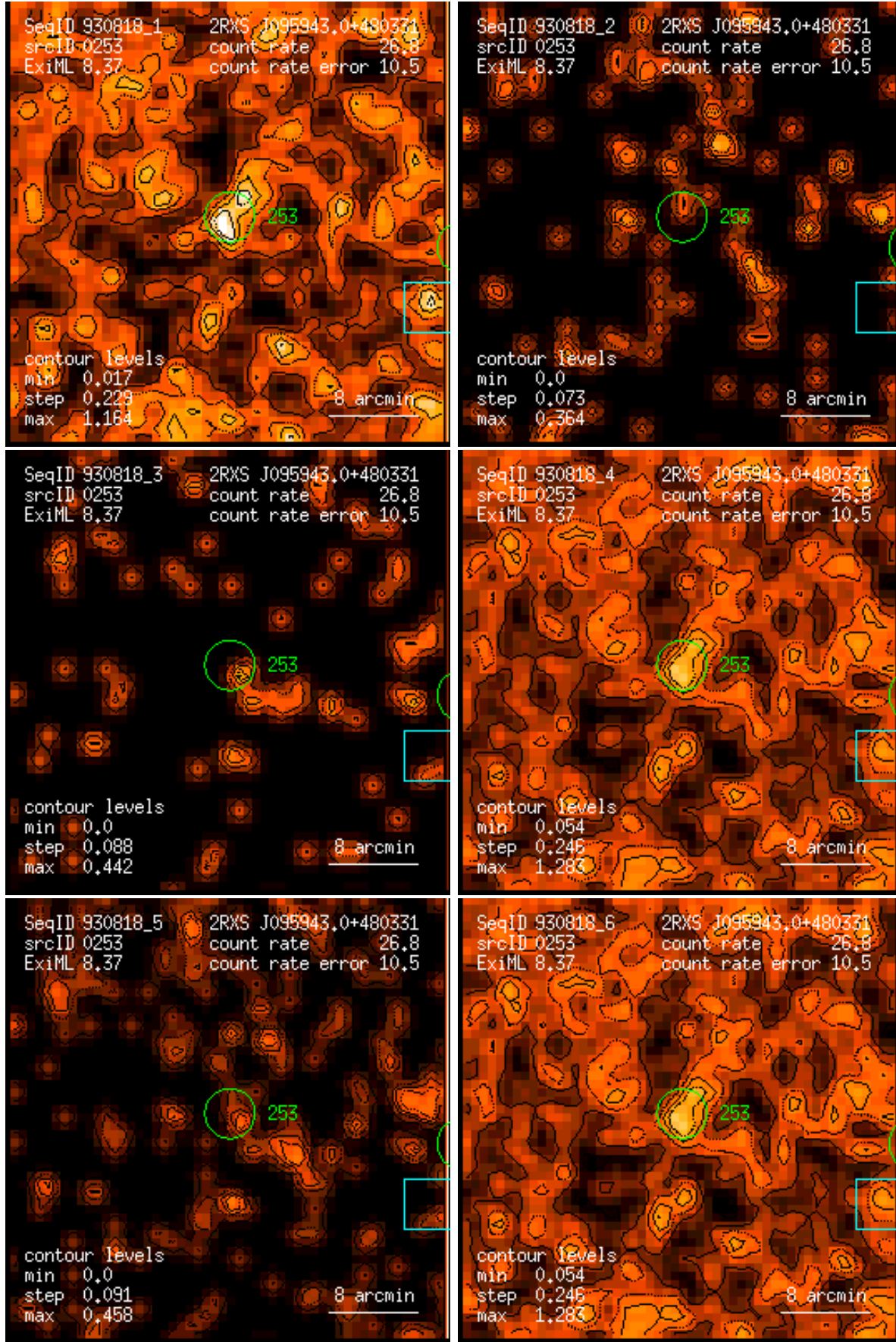
Figure 253: RASS 930818: detection 0253: band rate images, Gaussian filter: (1) PSPC channels 11 – 41, (2) 52 – 90, (3) 91 – 201, (4) 11 – 235, (5) 52 – 201, (6) 11 – 201. Broad band rates in counts/ks. Band rate contour levels in counts/ks/arcmin 2 .
