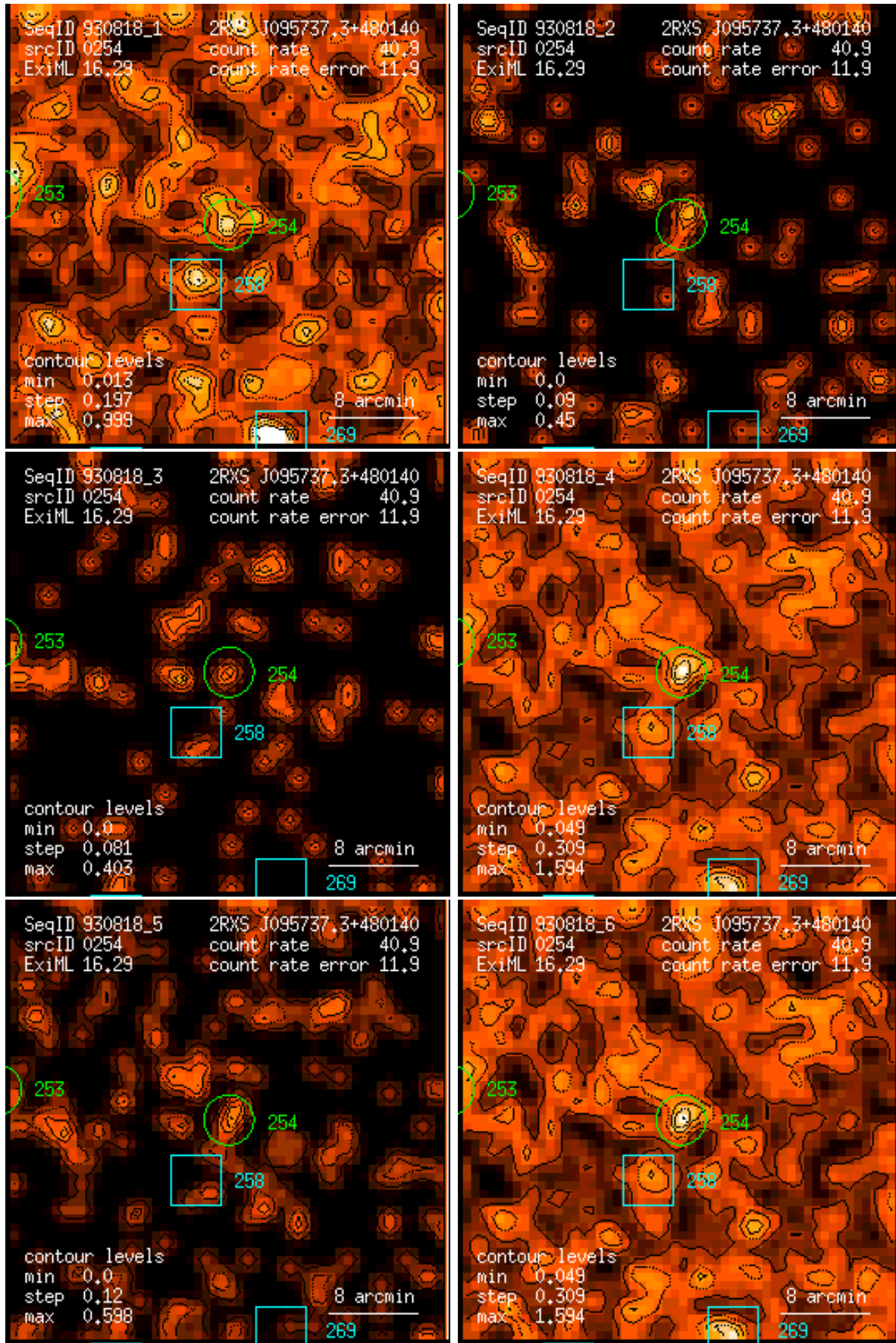
Figure 254: RASS 930818: detection 0254: band rate images, Gaussian filter: (1) PSPC channels 11 – 41, (2) 52 – 90, (3) 91 – 201, (4) 11 – 235, (5) 52 – 201, (6) 11 – 201. Broad band rates in counts/ks. Band rate contour levels in counts/ks/arcmin 2 .
