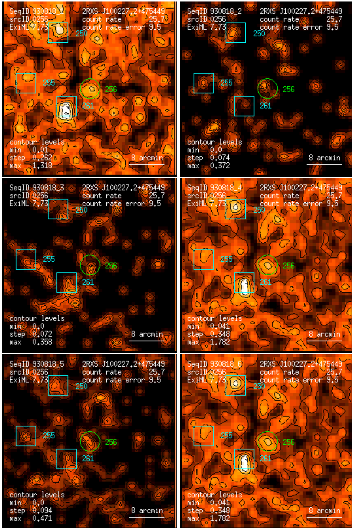
Figure 256: RASS 930818: detection 0256: band rate images, Gaussian filter: (1) PSPC channels 11 – 41, (2) 52 – 90, (3) 91 – 201, (4) 11 – 235, (5) 52 – 201, (6) 11 – 201. Broad band rates in counts/ks. Band rate contour levels in counts/ks/arcmin 2 .
