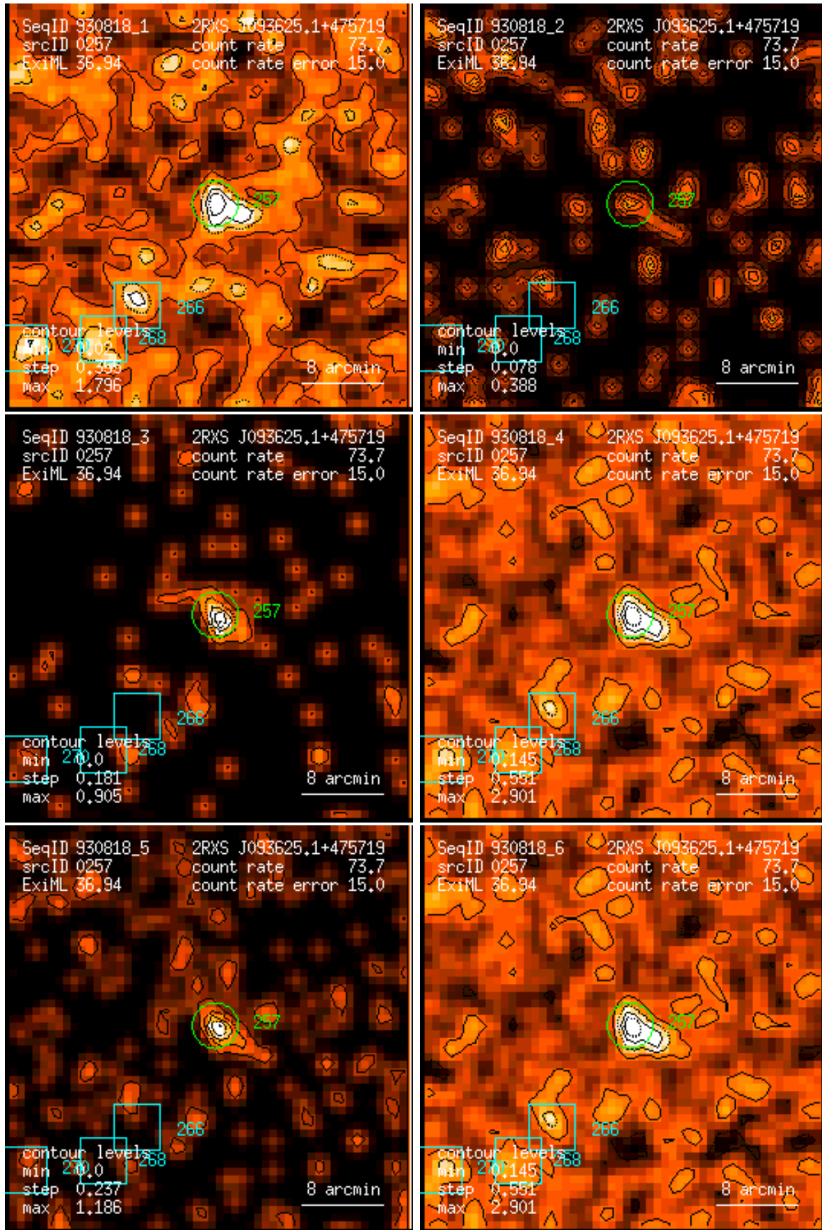
Figure 257: RASS 930818: detection 0257: band rate images, Gaussian filter: (1) PSPC channels 11 – 41, (2) 52 – 90, (3) 91 – 201, (4) 11 – 235, (5) 52 – 201, (6) 11 – 201. Broad band rates in counts/ks. Band rate contour levels in counts/ks/arcmin 2 .
