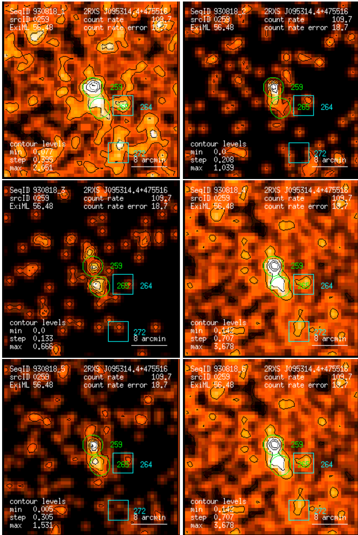
Figure 259: RASS 930818: detection 0259: band rate images, Gaussian filter: (1) PSPC channels 11 – 41, (2) 52 – 90, (3) 91 – 201, (4) 11 – 235, (5) 52 – 201, (6) 11 – 201. Broad band rates in counts/ks. Band rate contour levels in counts/ks/arcmin 2 .
