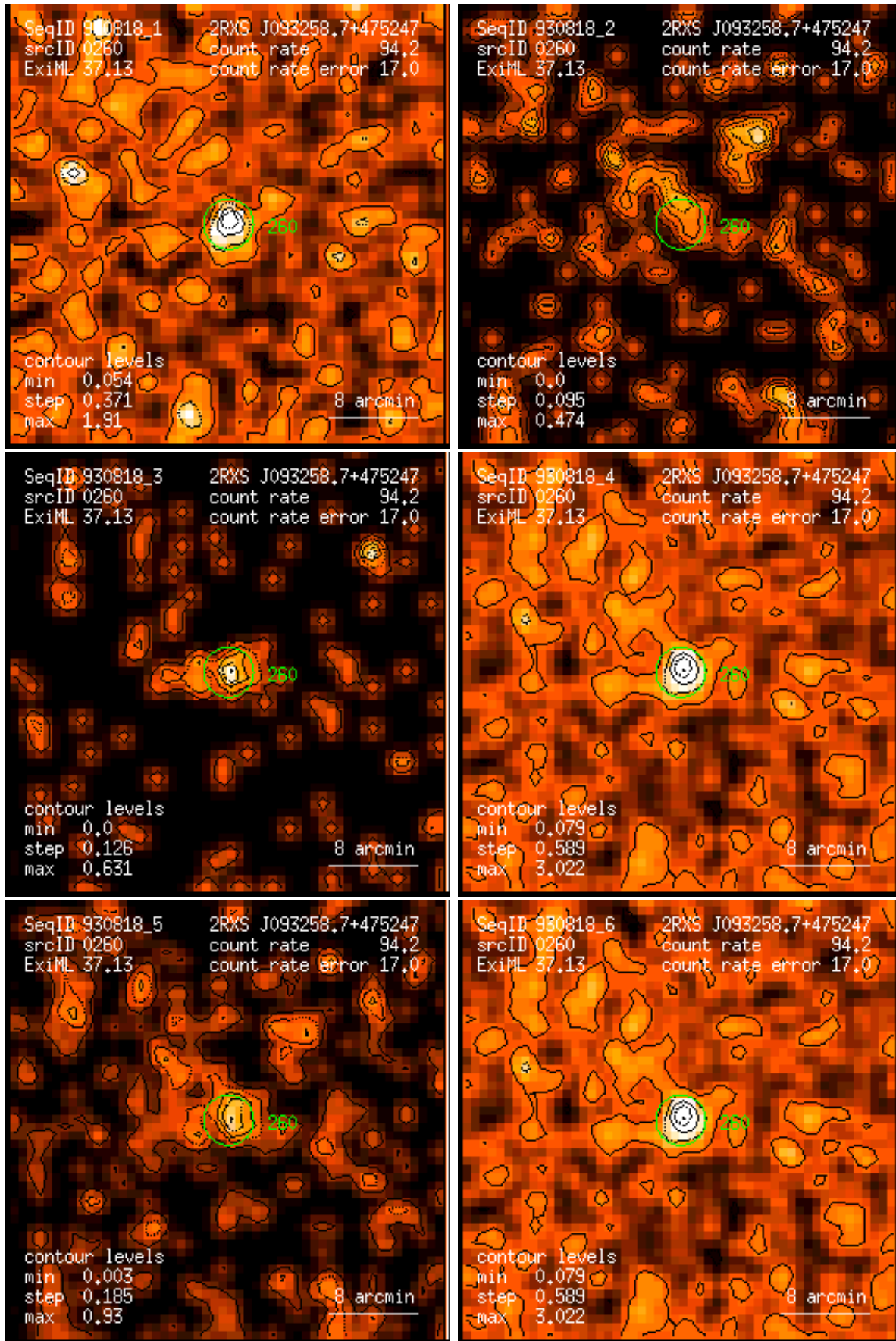
Figure 260: RASS 930818: detection 0260: band rate images, Gaussian filter: (1) PSPC channels 11 – 41, (2) 52 – 90, (3) 91 – 201, (4) 11 – 235, (5) 52 – 201, (6) 11 – 201. Broad band rates in counts/ks. Band rate contour levels in counts/ks/arcmin 2 .
