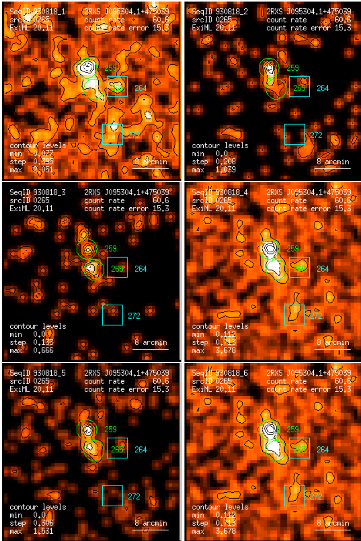
Figure 265: RASS 930818: detection 0265: band rate images, Gaussian filter: (1) PSPC channels 11 – 41, (2) 52 – 90, (3) 91 – 201, (4) 11 – 235, (5) 52 – 201, (6) 11 – 201. Broad band rates in counts/ks. Band rate contour levels in counts/ks/arcmin 2 .
