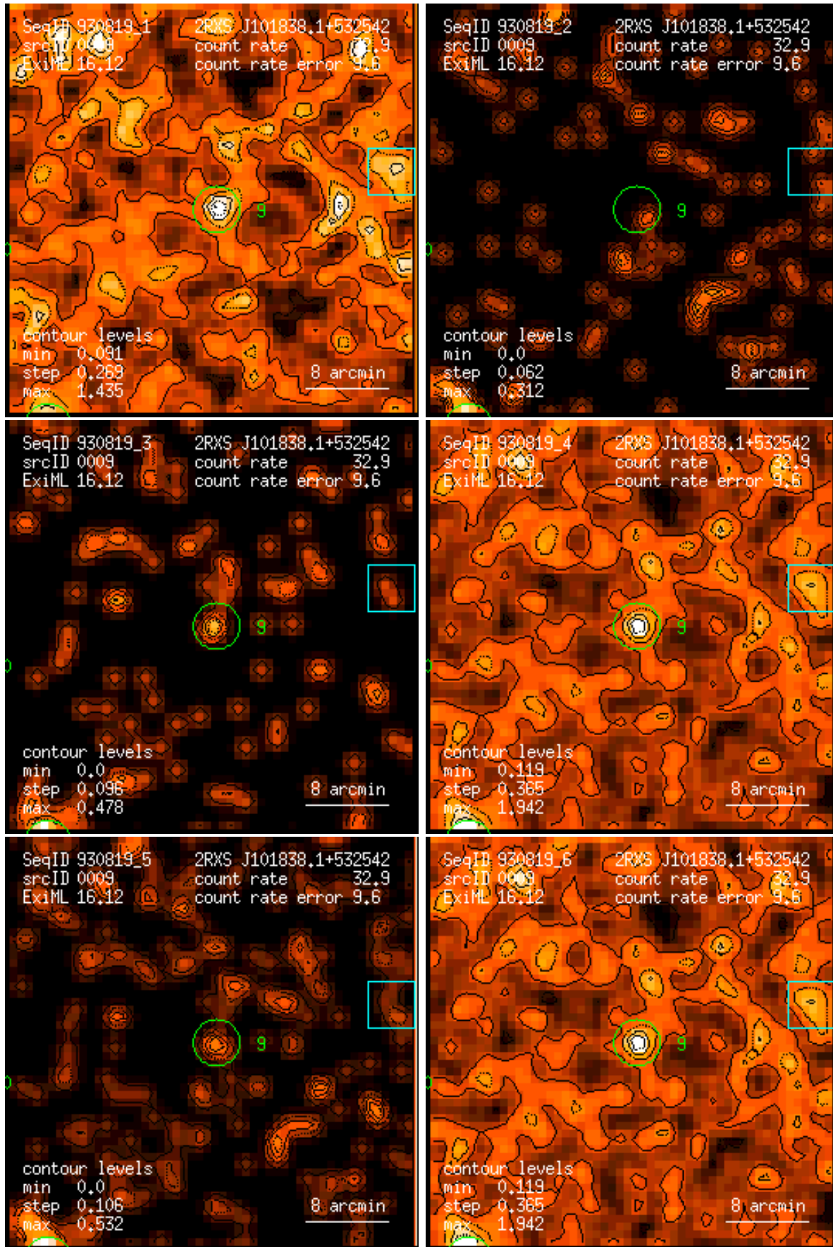
Figure 9: RASS 930819: detection 0009: band rate images, Gaussian filter: (1) PSPC channels 11 – 41, (2) 52 – 90, (3) 91 – 201, (4) 11 – 235, (5) 52 – 201, (6) 11 – 201. Broad band rates in counts/ks. Band rate contour levels in counts/ks/arcmin 2 .
