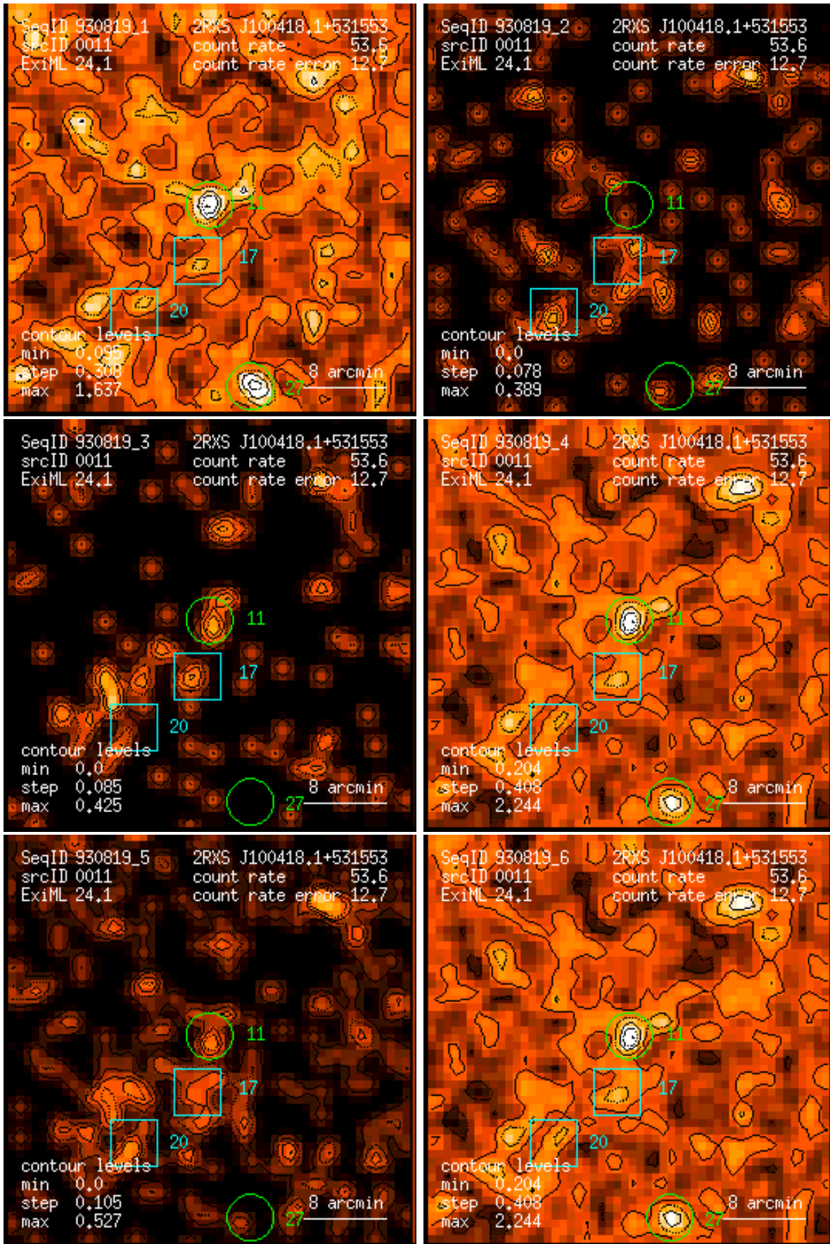
Figure 11: RASS 930819: detection 0011: band rate images, Gaussian filter: (1) PSPC channels 11 – 41, (2) 52 – 90, (3) 91 – 201, (4) 11 – 235, (5) 52 – 201, (6) 11 – 201. Broad band rates in counts/ks. Band rate contour levels in counts/ks/arcmin 2 .
