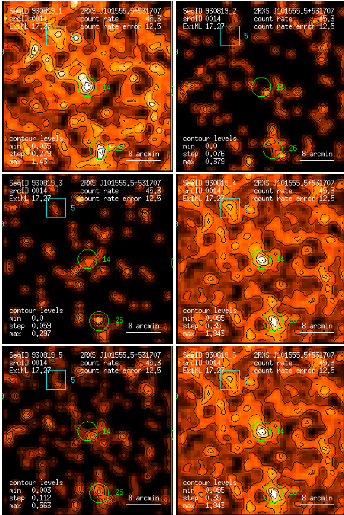
Figure 14: RASS 930819: detection 0014: band rate images, Gaussian filter: (1) PSPC channels 11 – 41, (2) 52 – 90, (3) 91 – 201, (4) 11 – 235, (5) 52 – 201, (6) 11 – 201. Broad band rates in counts/ks. Band rate contour levels in counts/ks/arcmin 2 .
