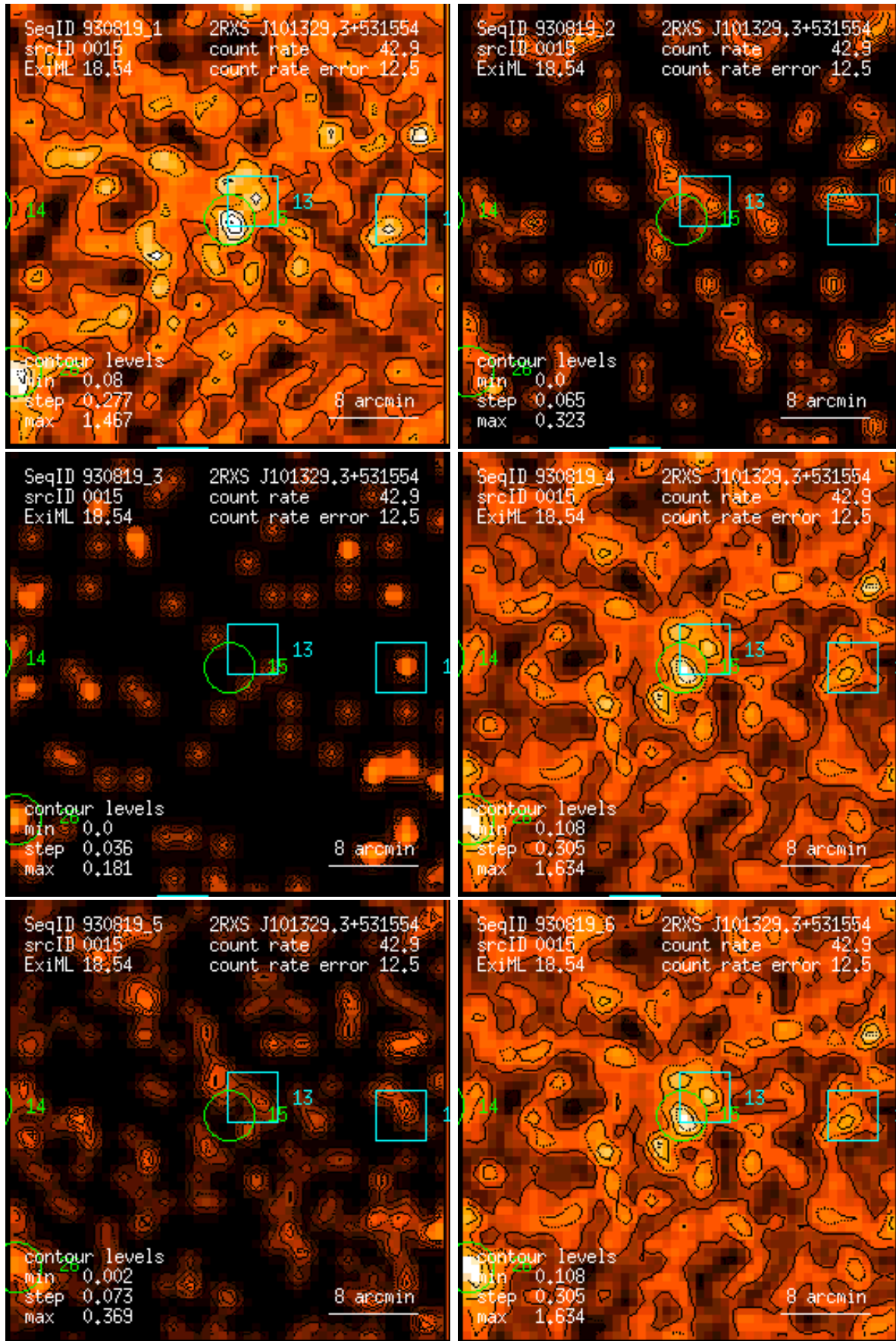
Figure 15: RASS 930819: detection 0015: band rate images, Gaussian filter: (1) PSPC channels 11 – 41, (2) 52 – 90, (3) 91 – 201, (4) 11 – 235, (5) 52 – 201, (6) 11 – 201. Broad band rates in counts/ks. Band rate contour levels in counts/ks/arcmin 2 .
