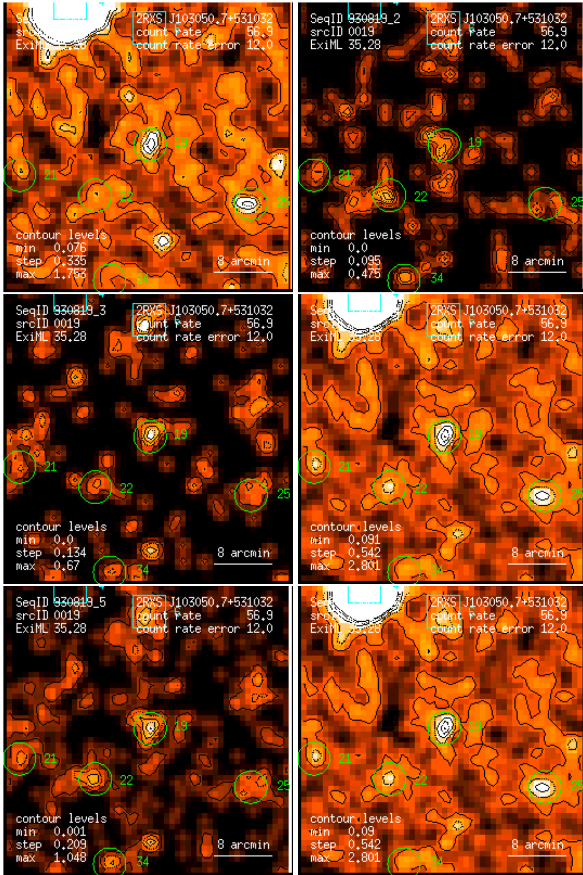
Figure 19: RASS 930819: detection 0019: band rate images, Gaussian filter: (1) PSPC channels 11 – 41, (2) 52 – 90, (3) 91 – 201, (4) 11 – 235, (5) 52 – 201, (6) 11 – 201. Broad band rates in counts/ks. Band rate contour levels in counts/ks/arcmin 2 .
