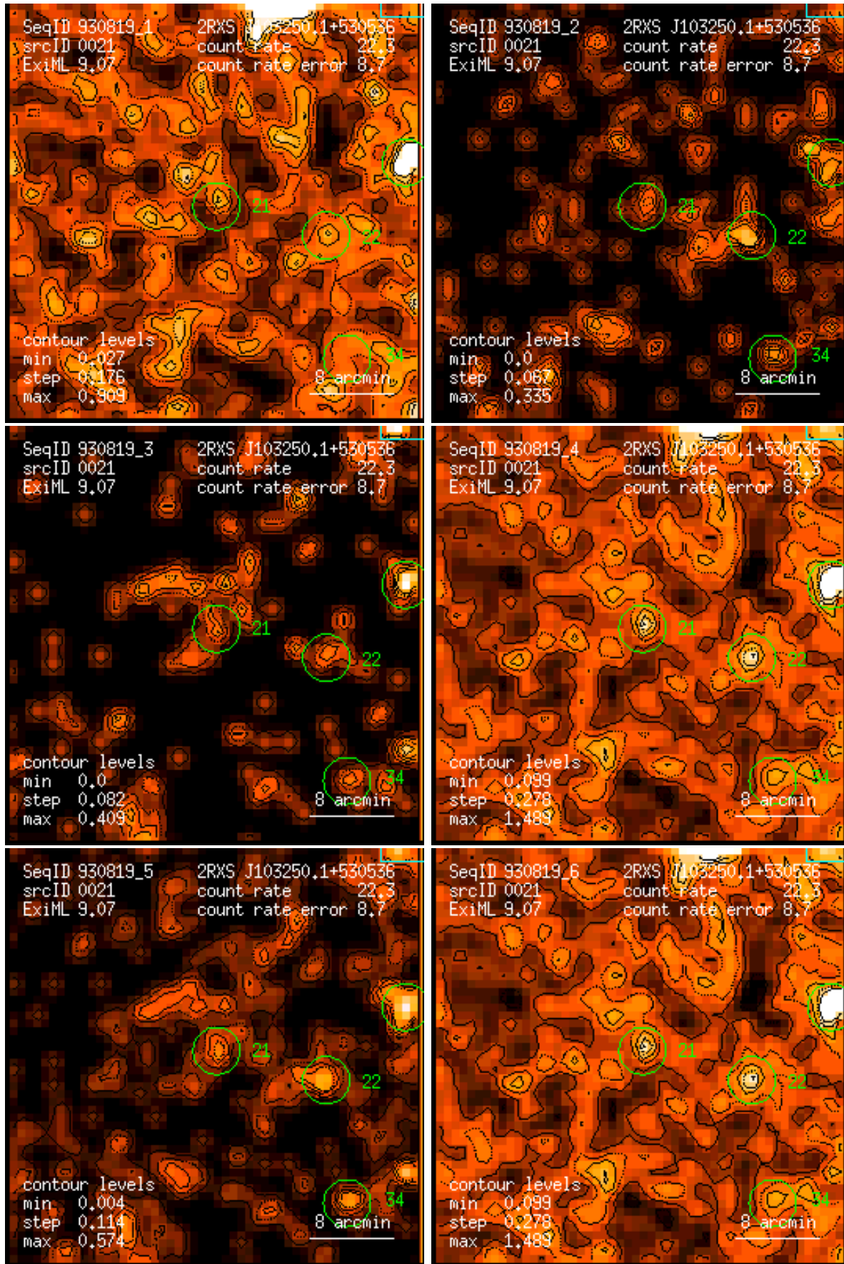
Figure 21: RASS 930819: detection 0021: band rate images, Gaussian filter: (1) PSPC channels 11 – 41, (2) 52 – 90, (3) 91 – 201, (4) 11 – 235, (5) 52 – 201, (6) 11 – 201. Broad band rates in counts/ks. Band rate contour levels in counts/ks/arcmin 2 .
