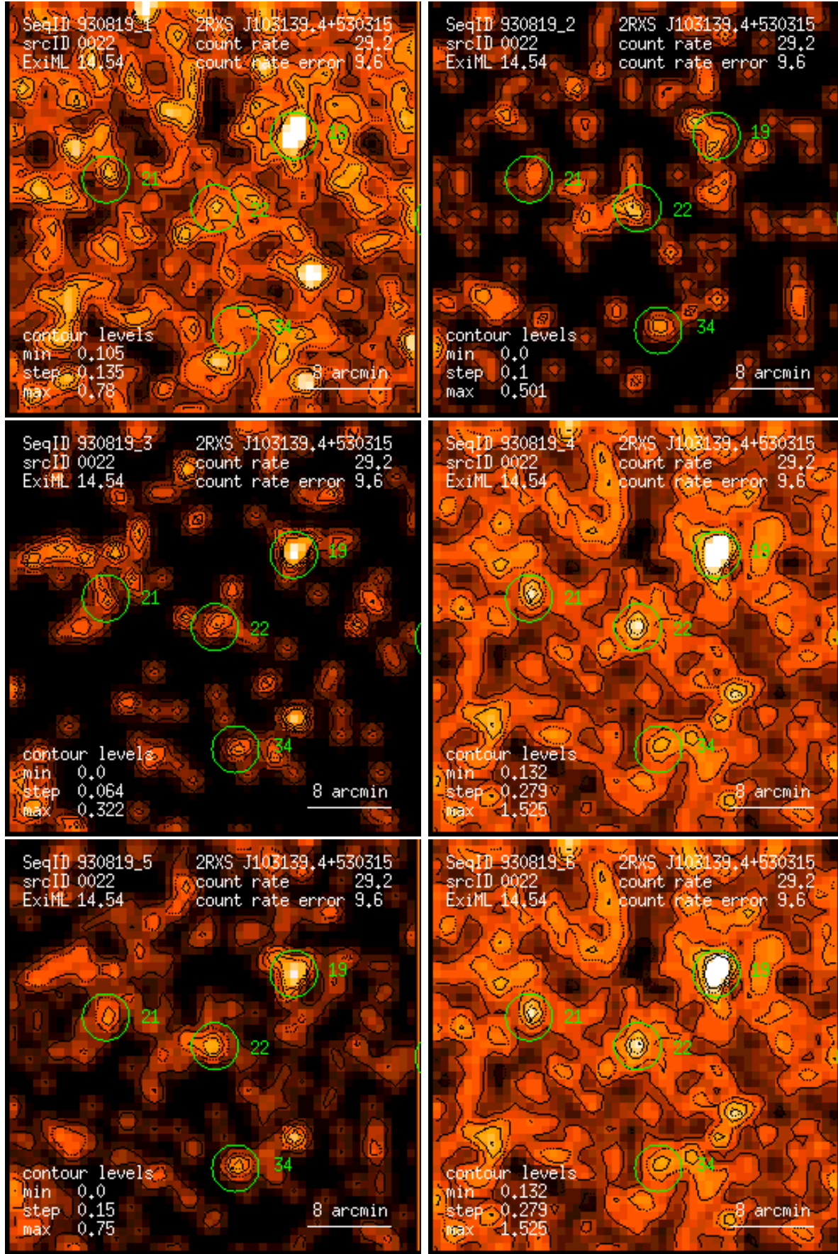
Figure 22: RASS 930819: detection 0022: band rate images, Gaussian filter: (1) PSPC channels 11 – 41, (2) 52 – 90, (3) 91 – 201, (4) 11 – 235, (5) 52 – 201, (6) 11 – 201. Broad band rates in counts/ks. Band rate contour levels in counts/ks/arcmin 2 .
