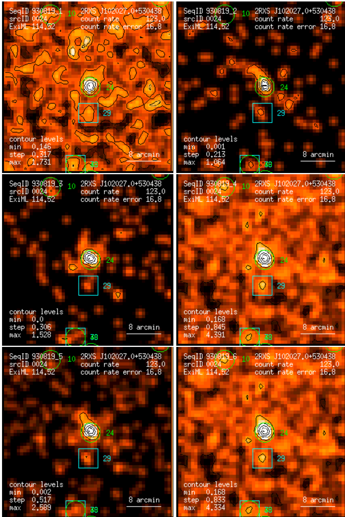
Figure 24: RASS 930819: detection 0024: band rate images, Gaussian filter: (1) PSPC channels 11 – 41, (2) 52 – 90, (3) 91 – 201, (4) 11 – 235, (5) 52 – 201, (6) 11 – 201. Broad band rates in counts/ks. Band rate contour levels in counts/ks/arcmin 2 .
