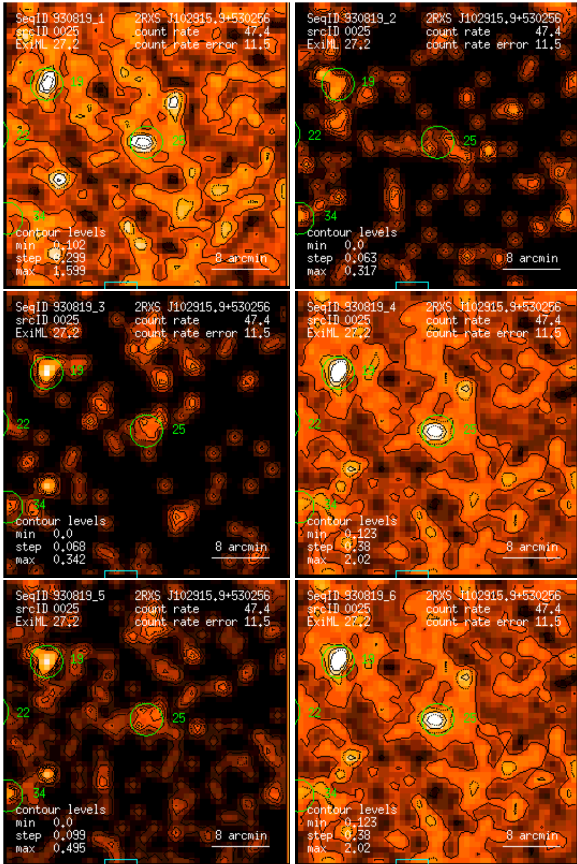
Figure 25: RASS 930819: detection 0025: band rate images, Gaussian filter: (1) PSPC channels 11 – 41, (2) 52 – 90, (3) 91 – 201, (4) 11 – 235, (5) 52 – 201, (6) 11 – 201. Broad band rates in counts/ks. Band rate contour levels in counts/ks/arcmin 2 .
